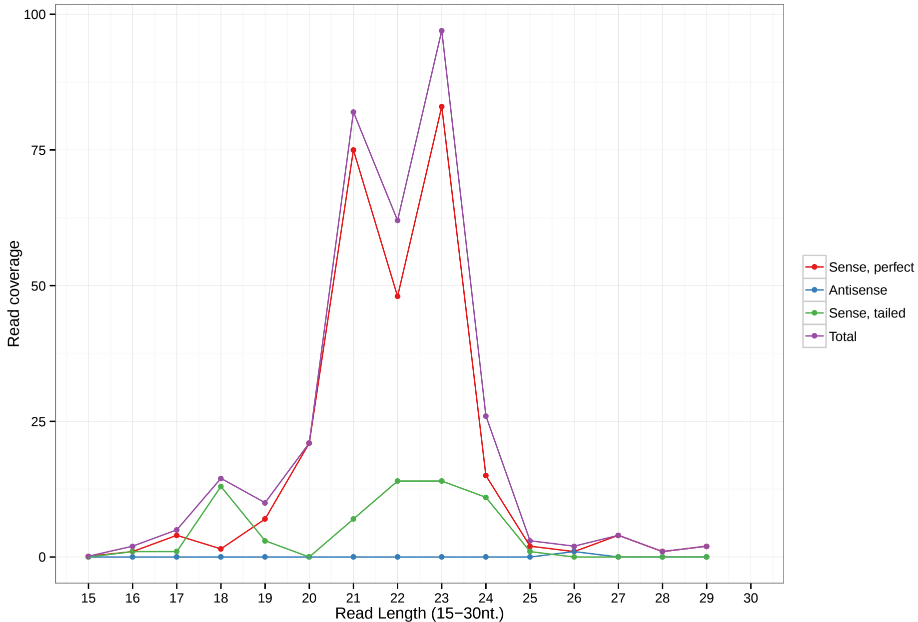
mmu-mir-6905
