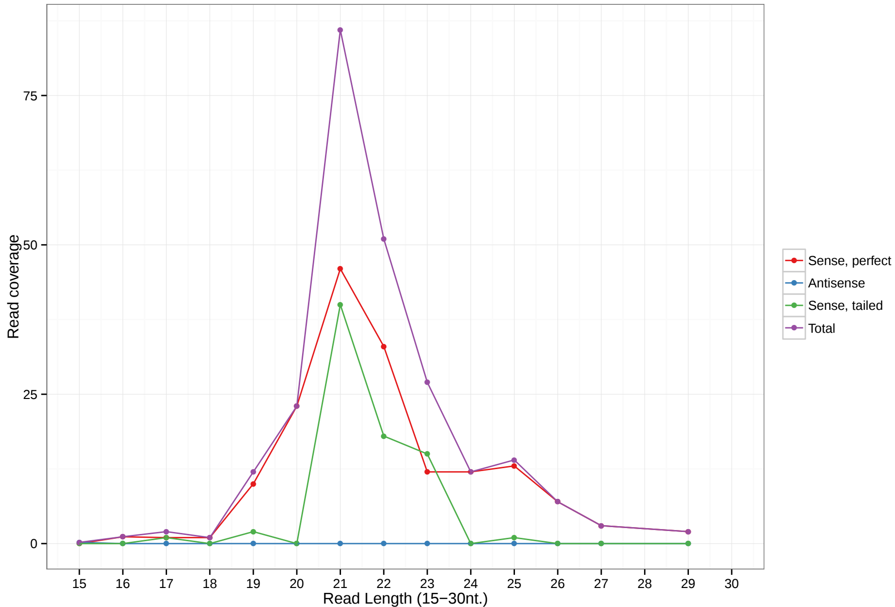
mmu-mir-6903
