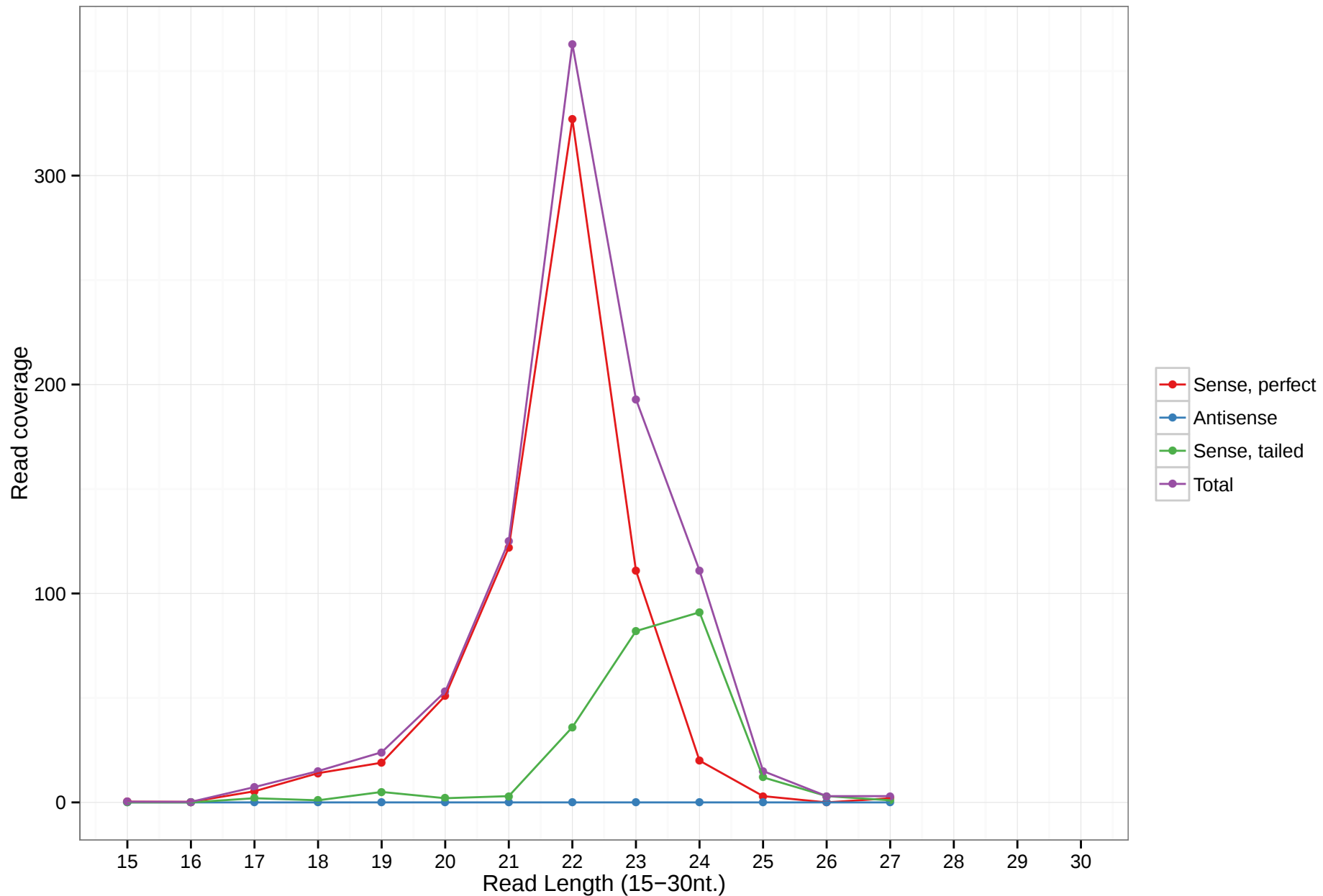
mmu-mir-6896
