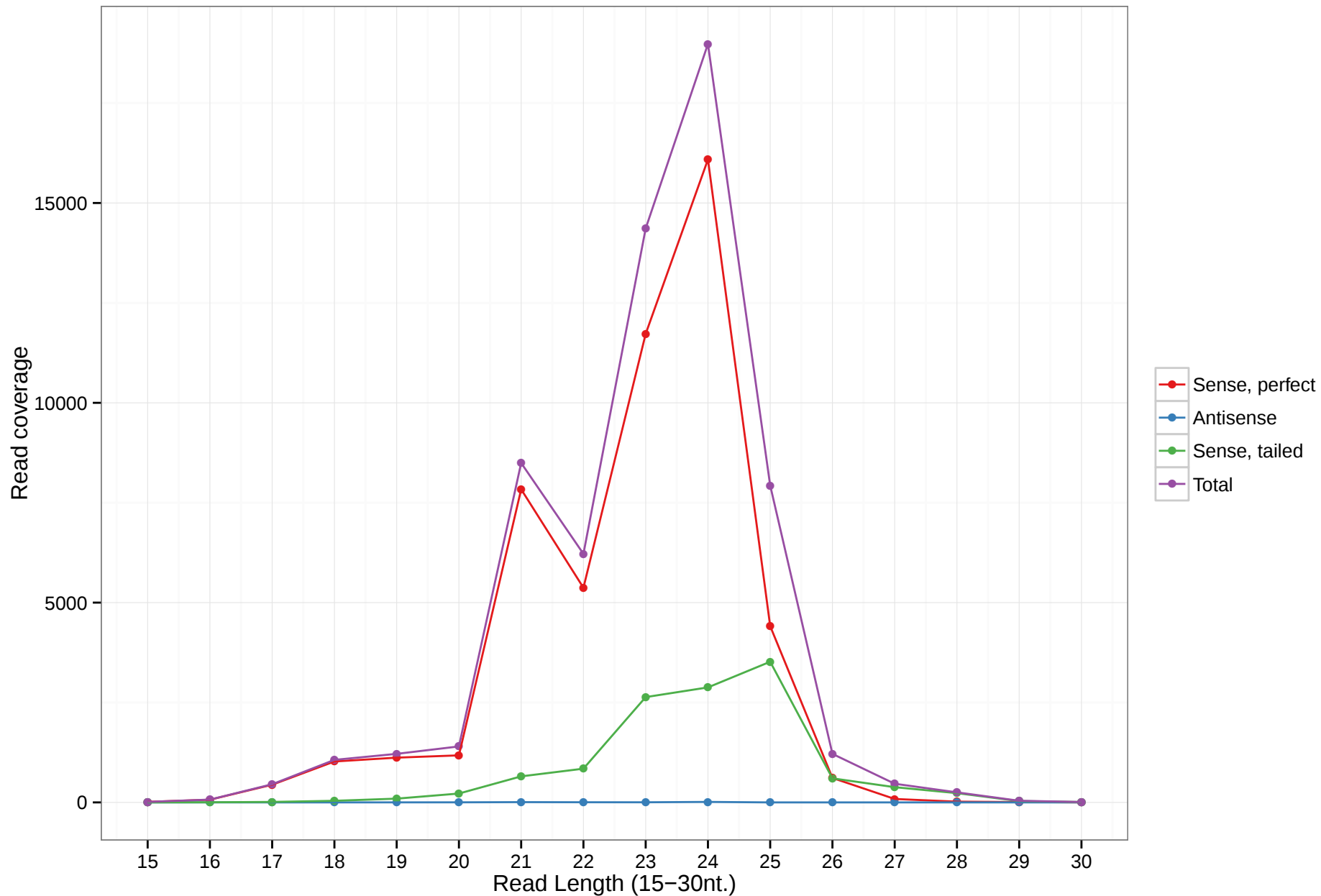
mmu-mir-668
