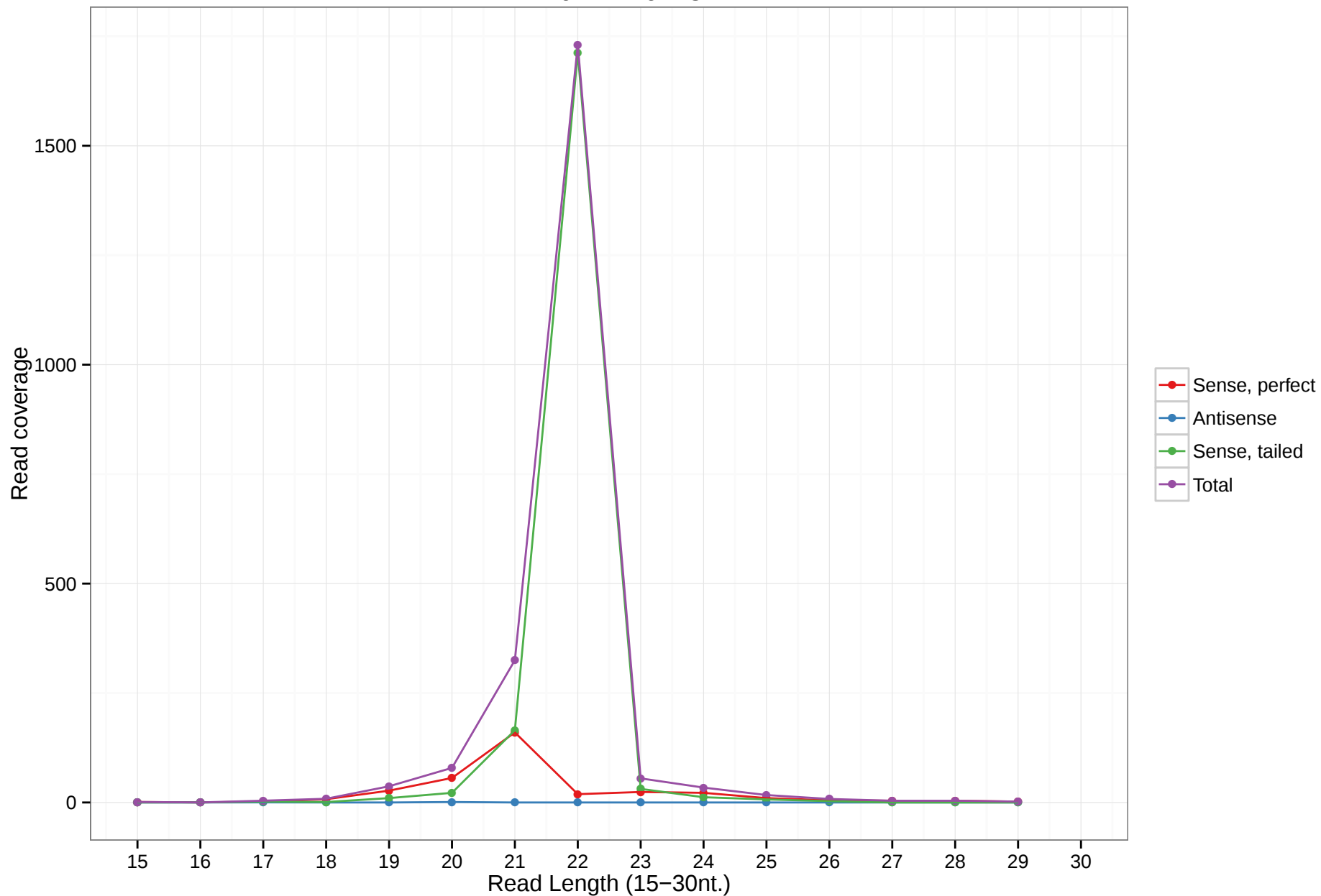
mmu-mir-6418
