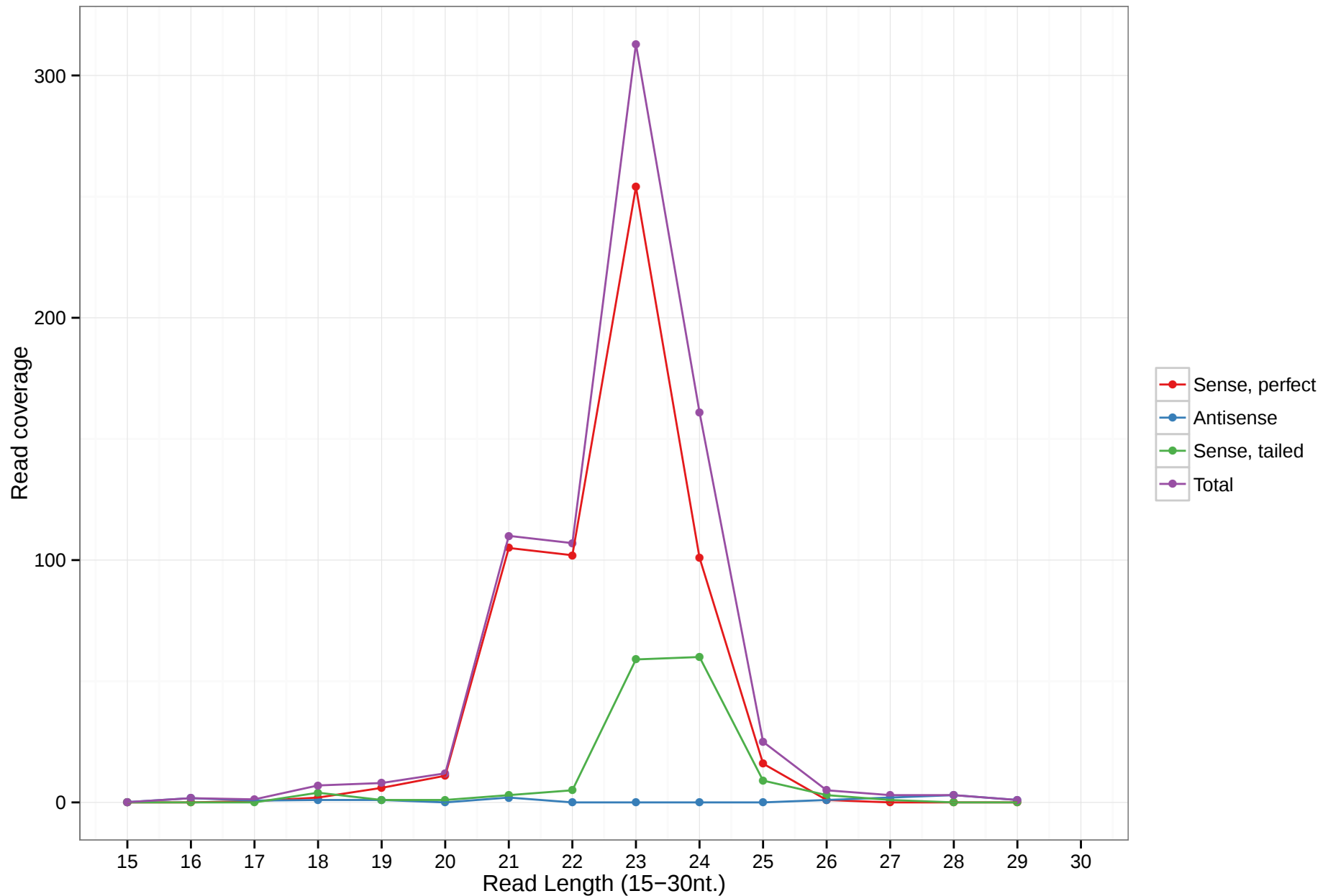
mmu-mir-5617
