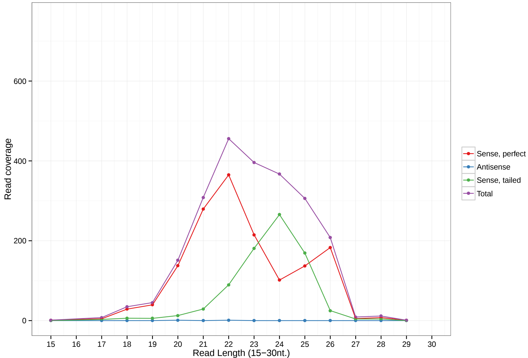
mmu-mir-3572
