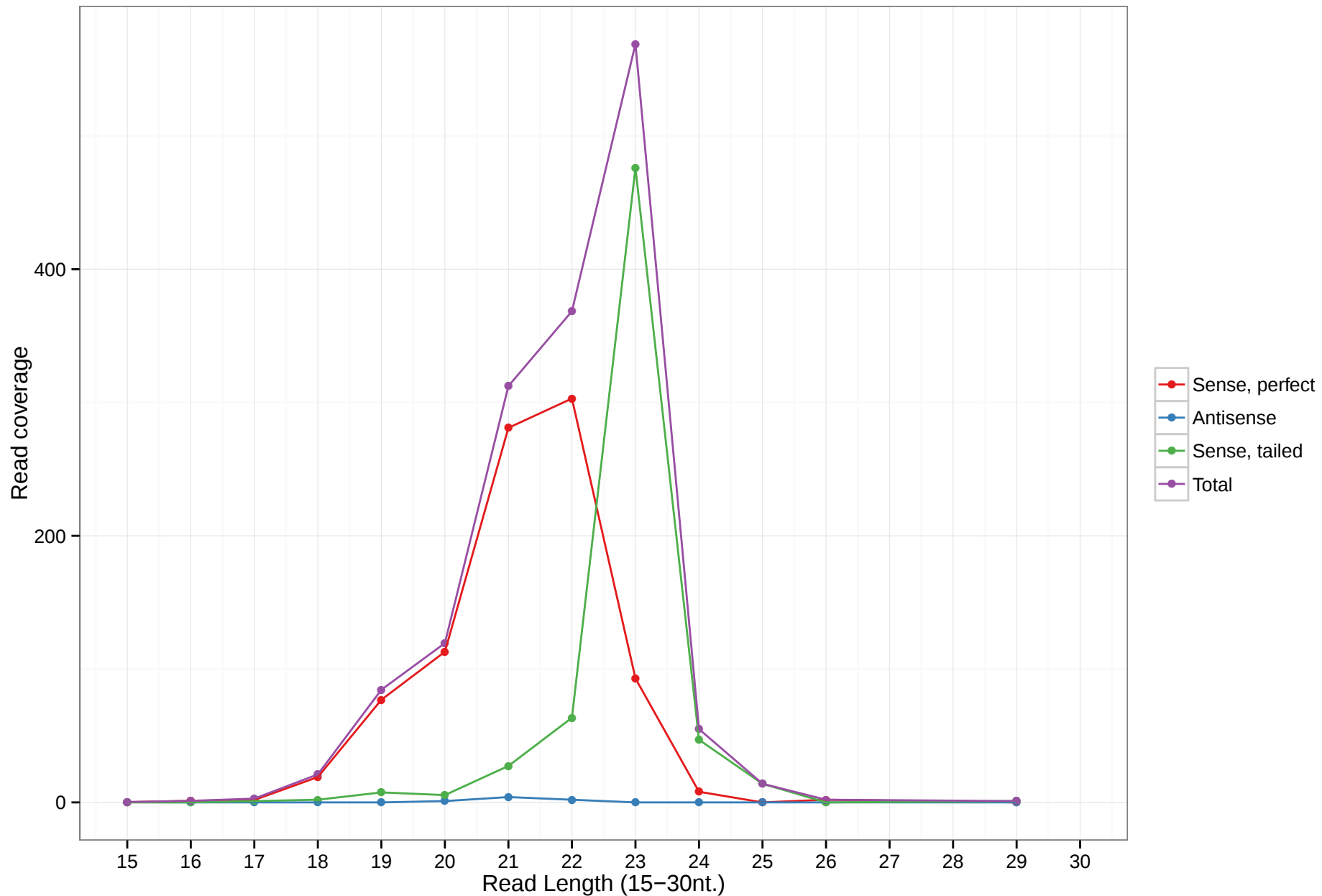
mmu-mir-3087
