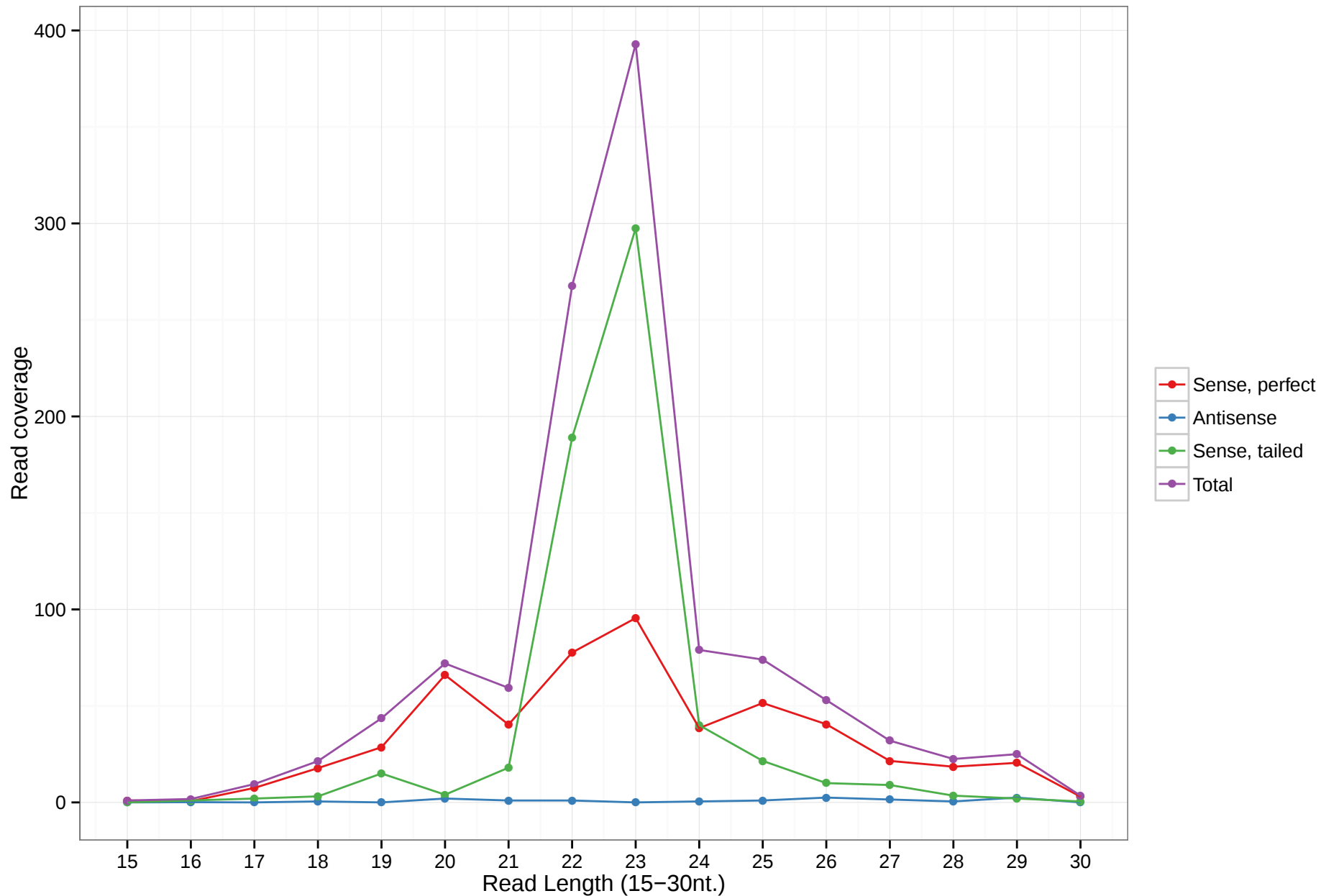
mmu-mir-3077
