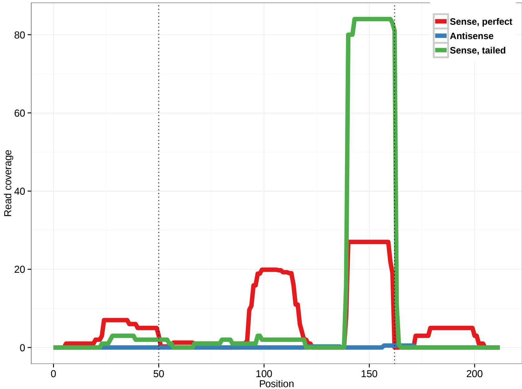
uc009iac.14
