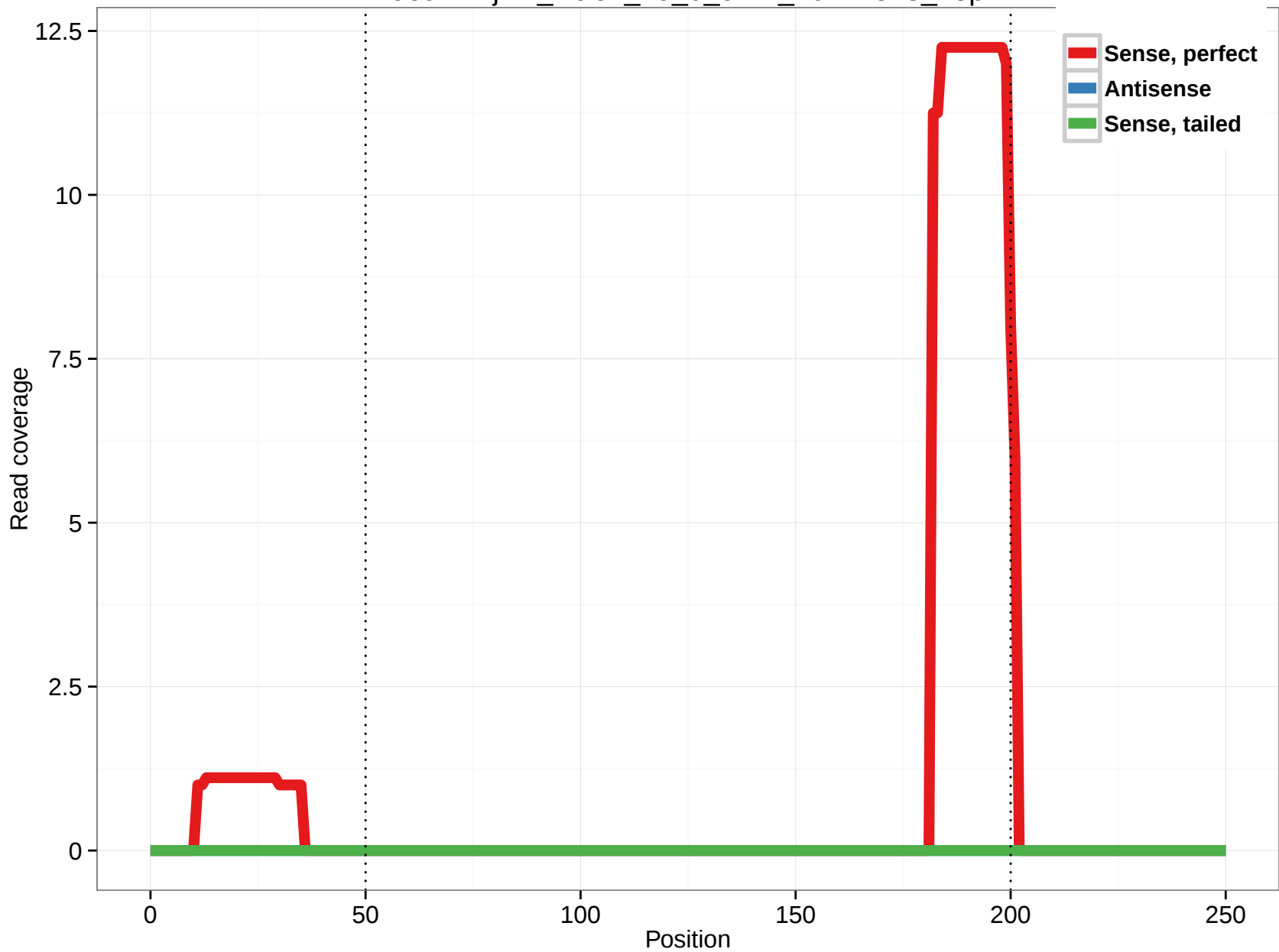
uc011mjk.1_intron_19_0_chrX_20227523_r.5p
