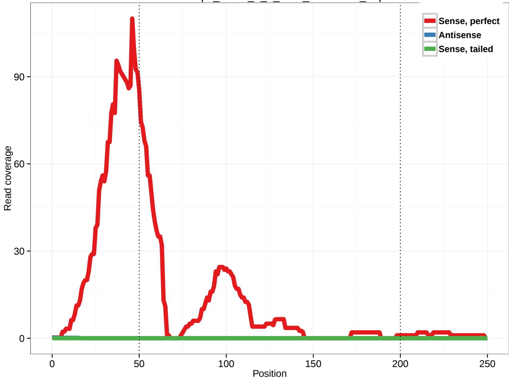
uc011miq.1_intron_3_0_chrX_15344169_r.5p
