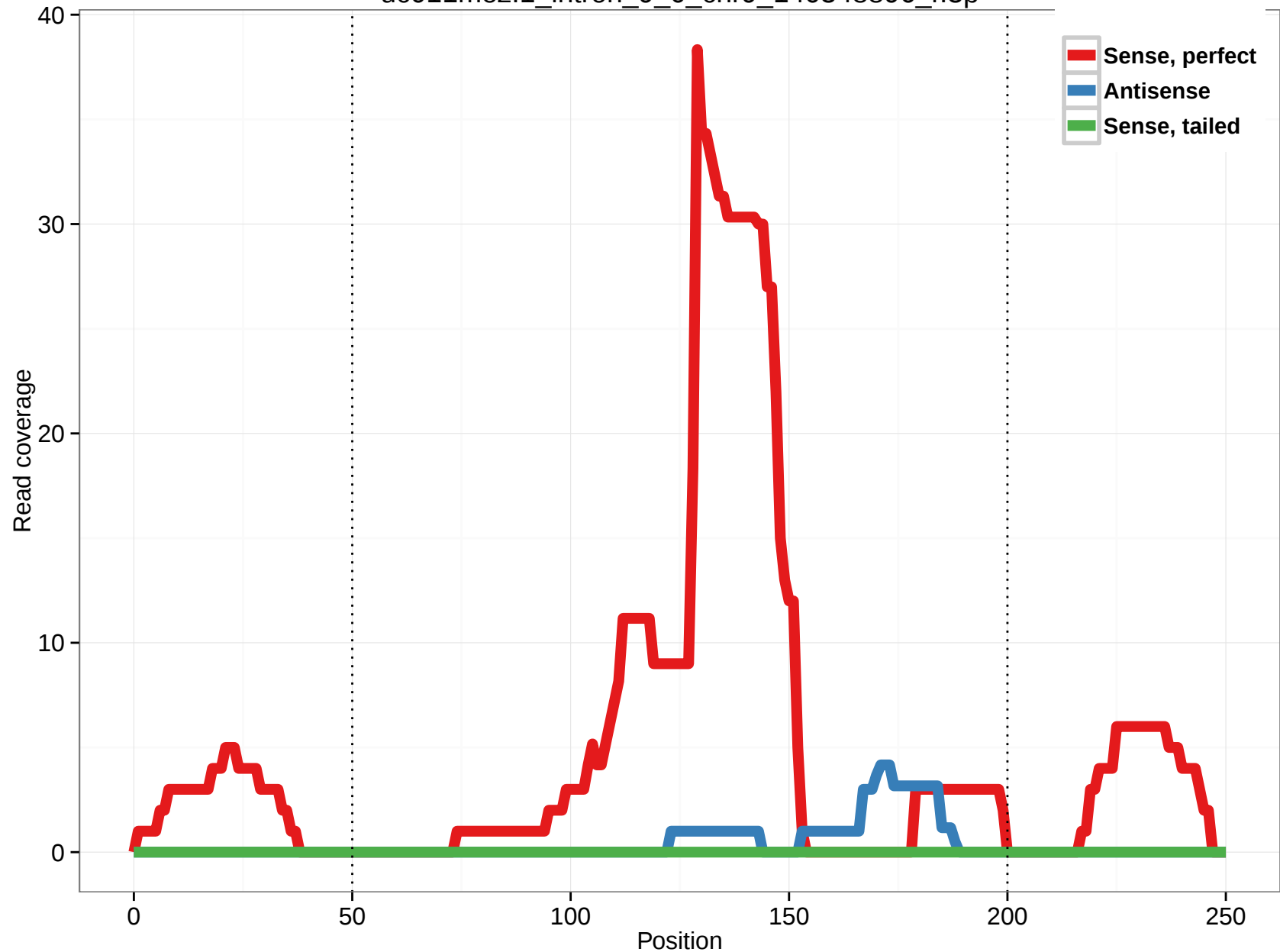
uc011mez.1_intron_9_0_chr9_140348896_r.3p
