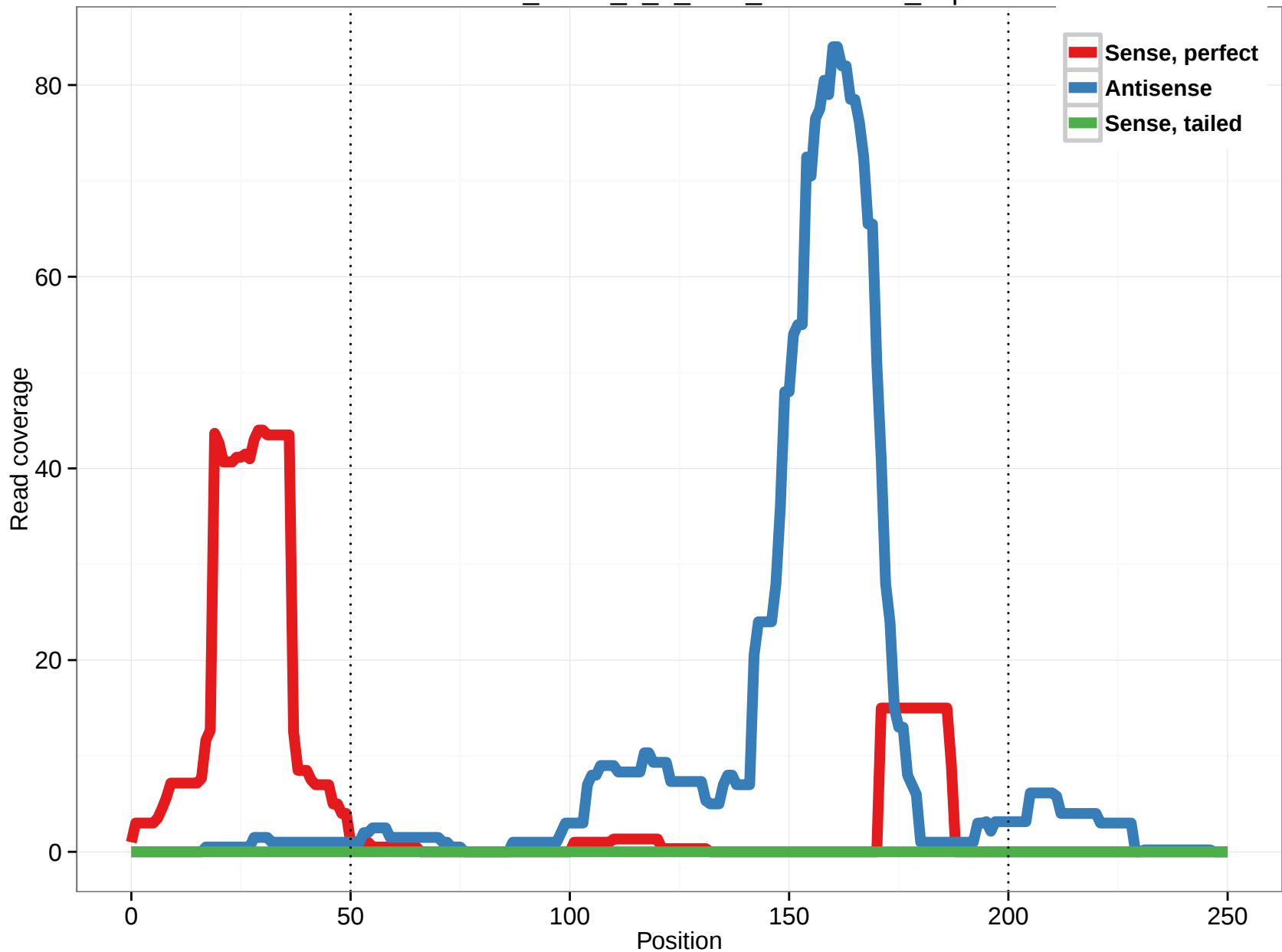
uc011lur.1_intron_0_0_chr9_100000850_f.5p
