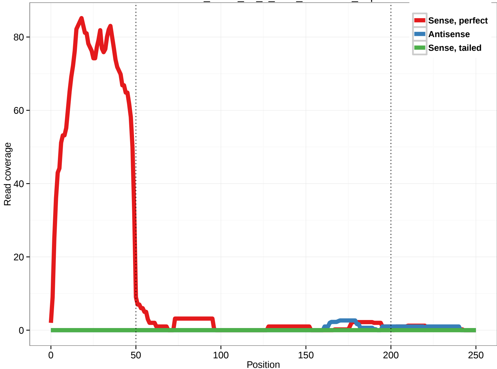
uc011loc.1_intron_18_0_chr9_33956145_r.5p
