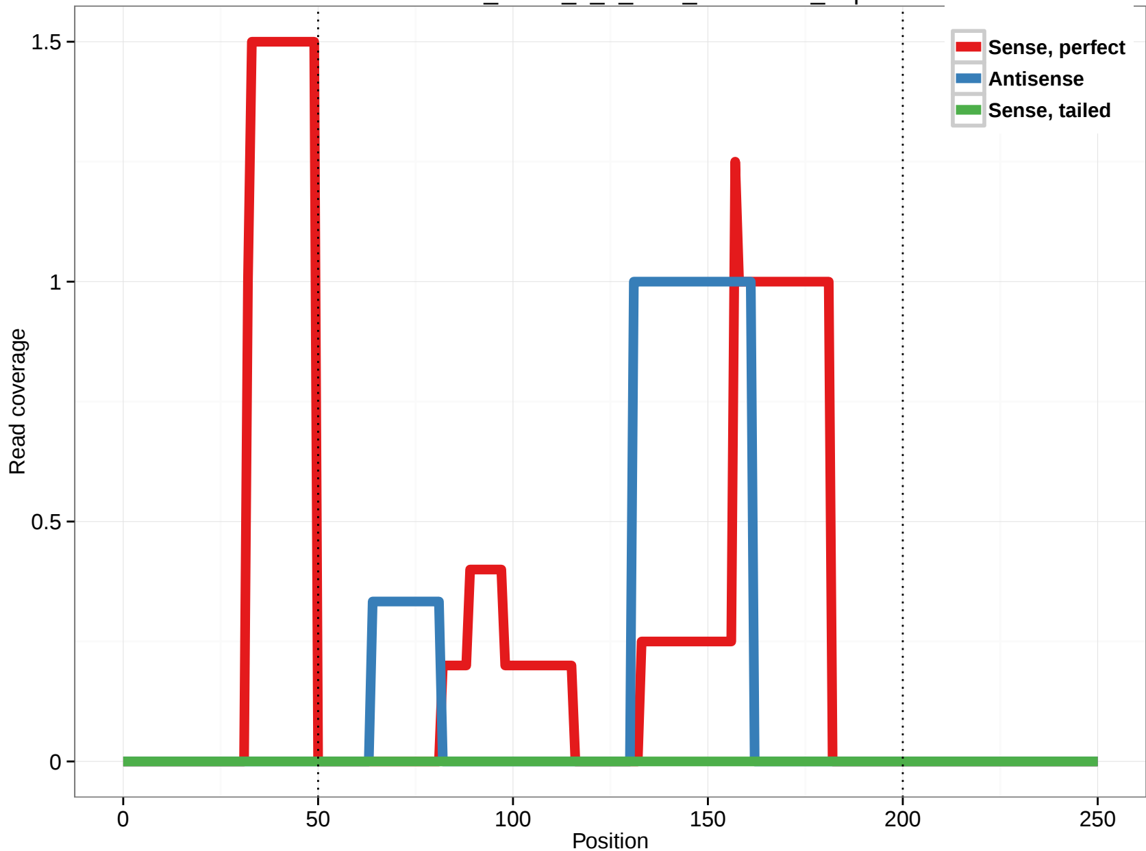
uc011lmz.1_intron_6_0_chr9_19076703_r.5p
