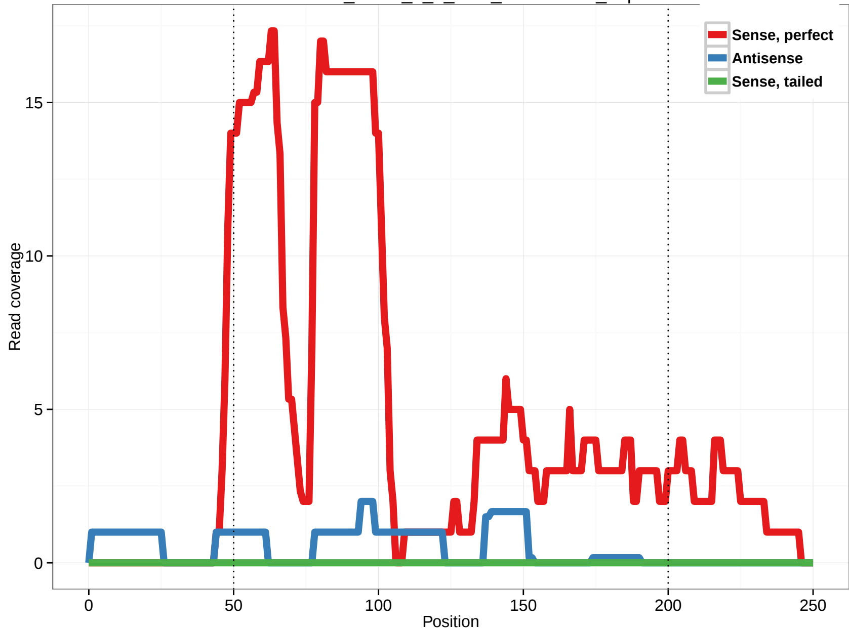
uc011li.1_intron_0_0_chr8_145728509_f.3p
