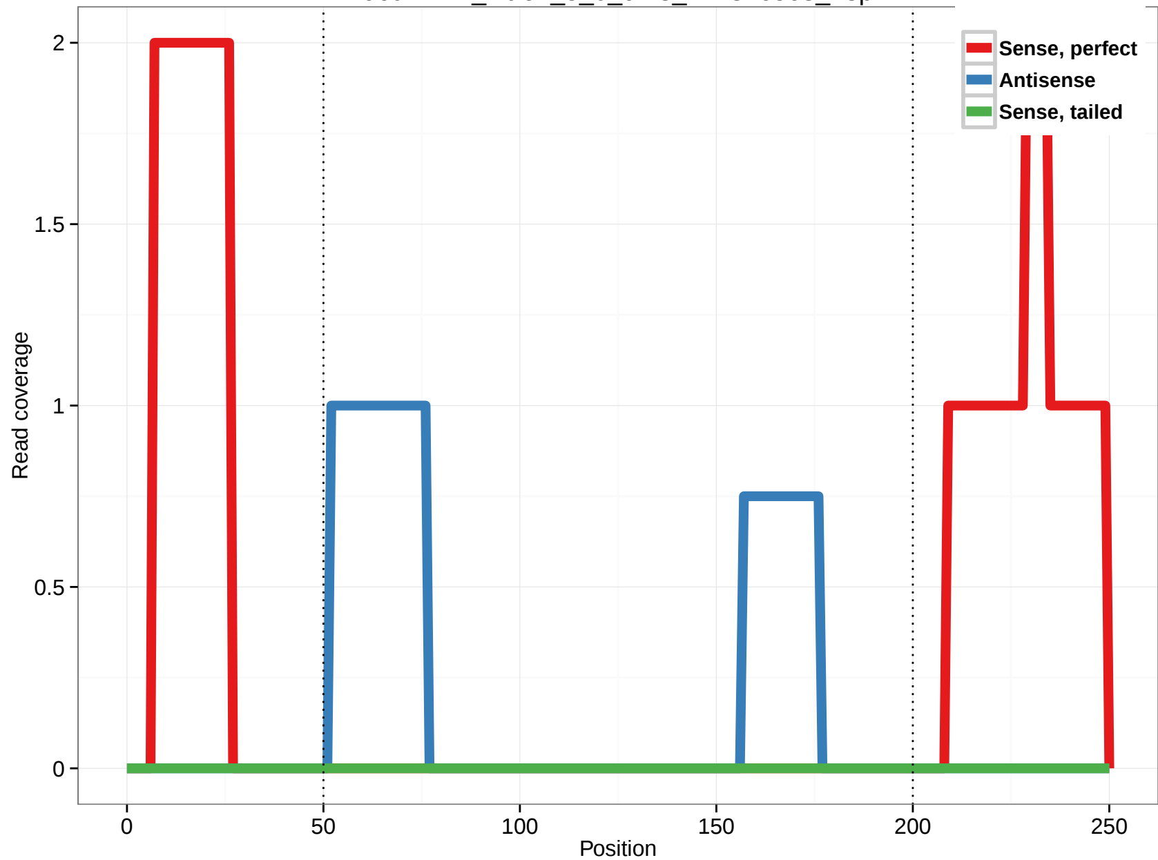
uc011lii.1_intron_5_0_chr8_124346563_r.3p
