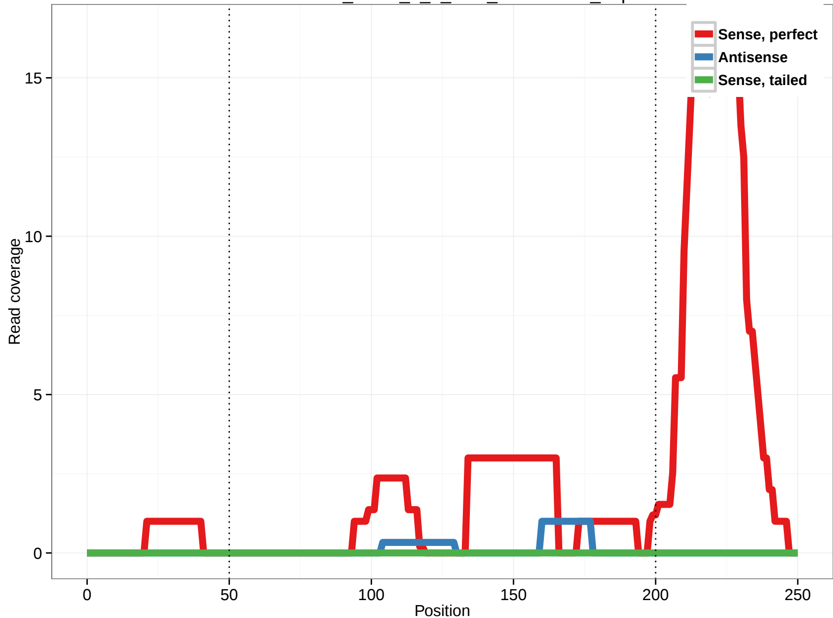
uc011lhk.1_intron_2_0_chr8_103664626_r.3p
