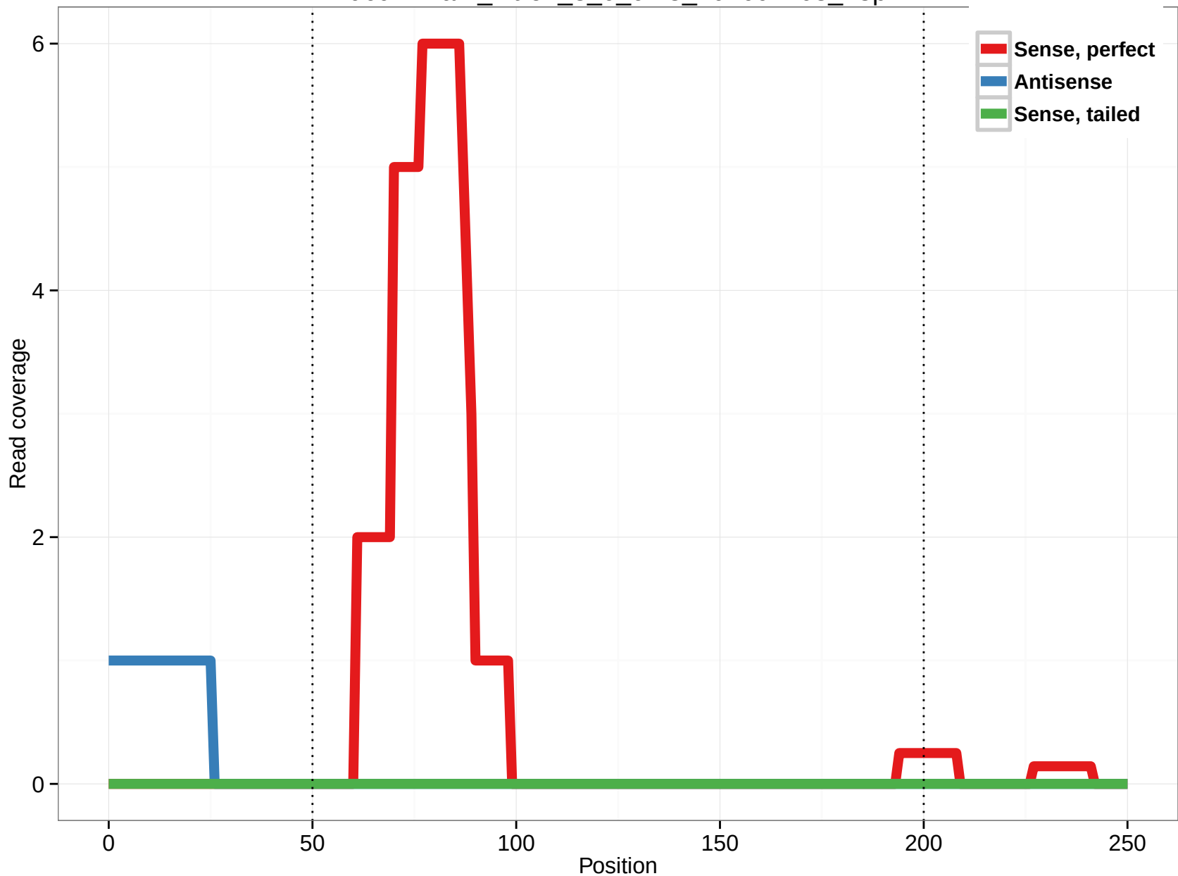
uc011lha.1_intron_3_0_chr8_101601208_r.3p
