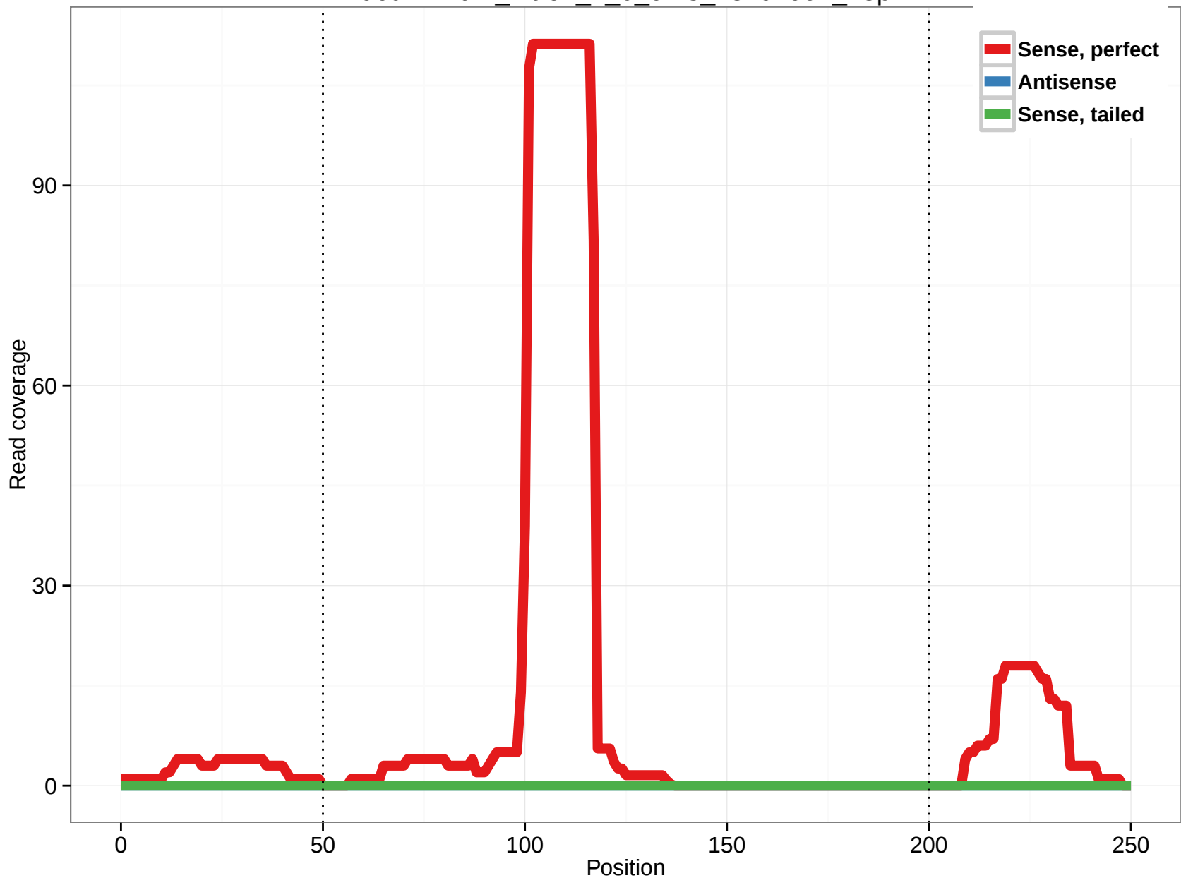
uc011kzu.1_intron_1_0_chr8_23291992_r.3p
