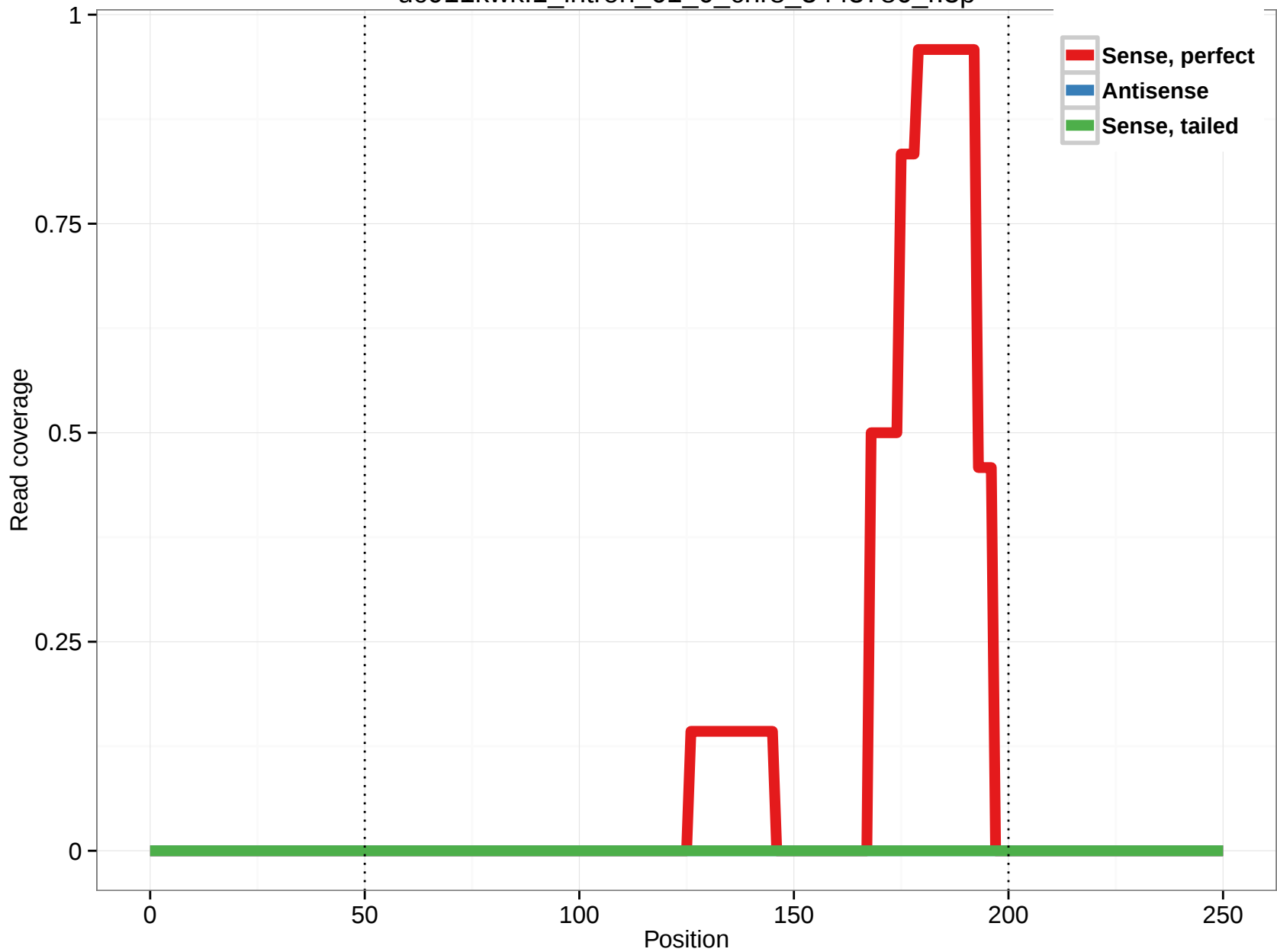
uc011kwk.1_intron_61_0_chr8_3443786_r.3p
