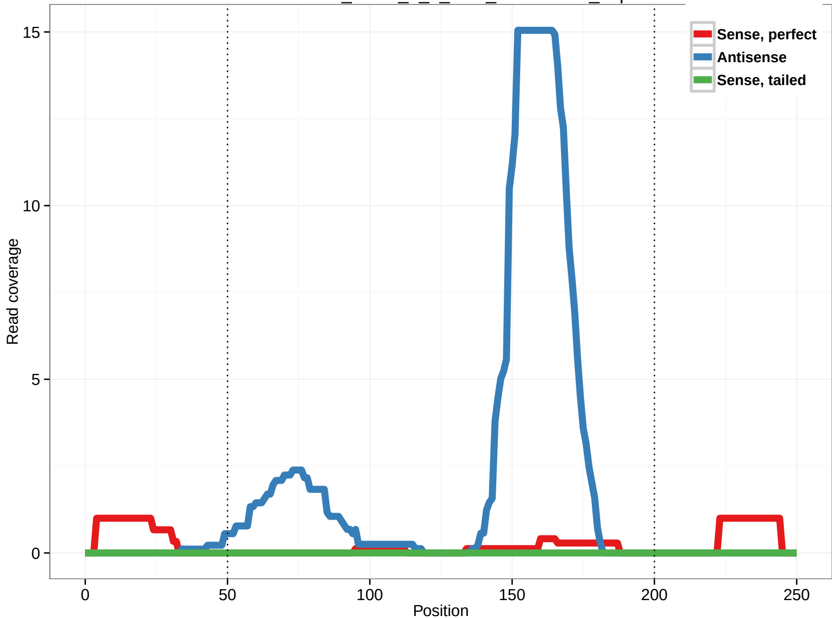
uc011kle.1_intron_4_0_chr7_102296754_f.5p
