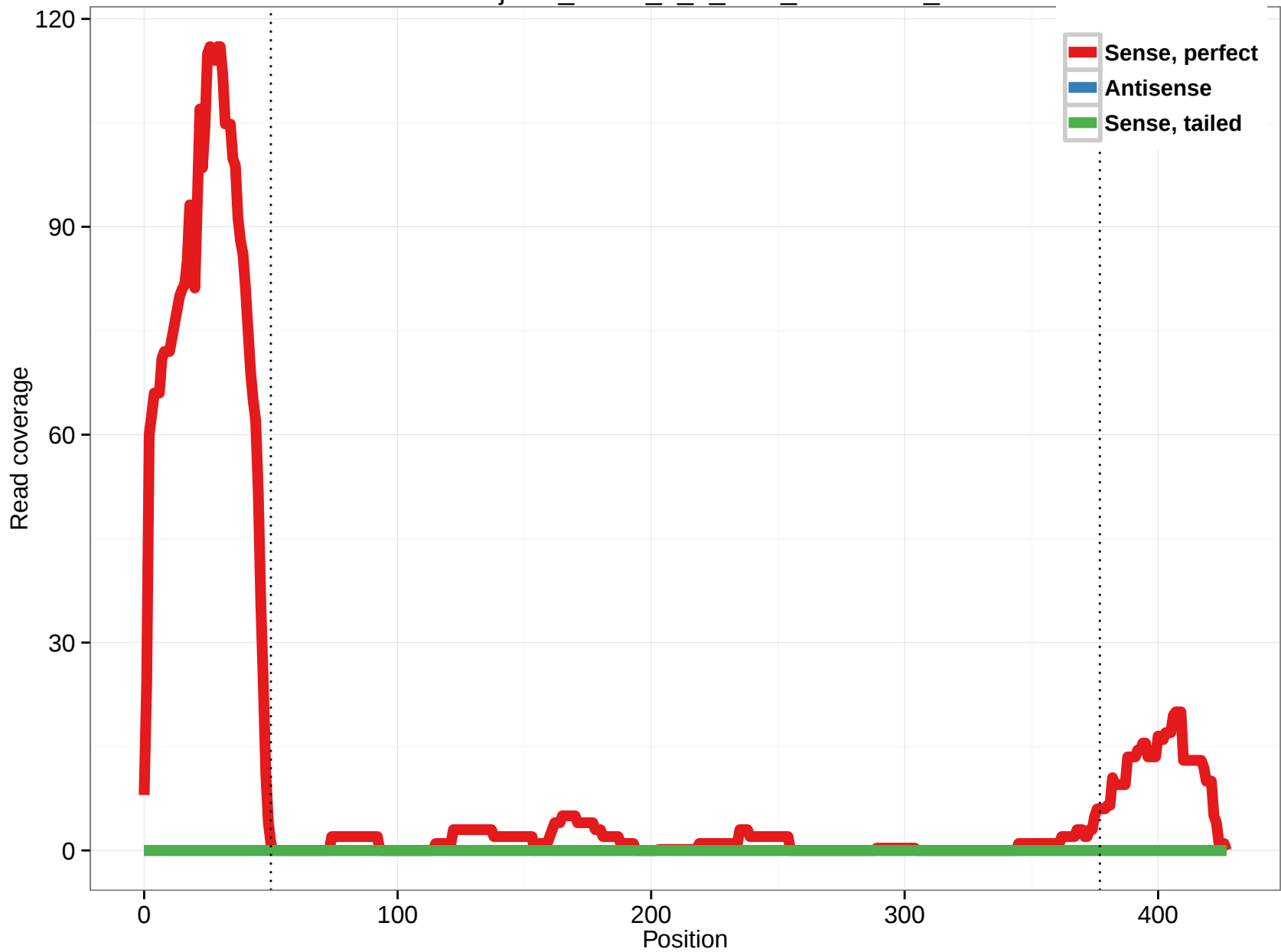
uc011jzb.1_intron_1_0_chr7_23545430_r
