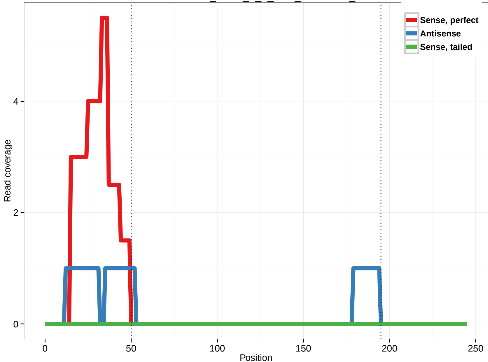
uc011dne.1_intron_5_0_chr6_31113080_r
