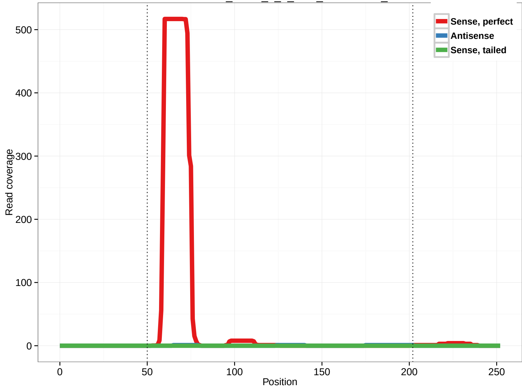
uc011dhi.1_intron_3_0_chr5_180480317_f
