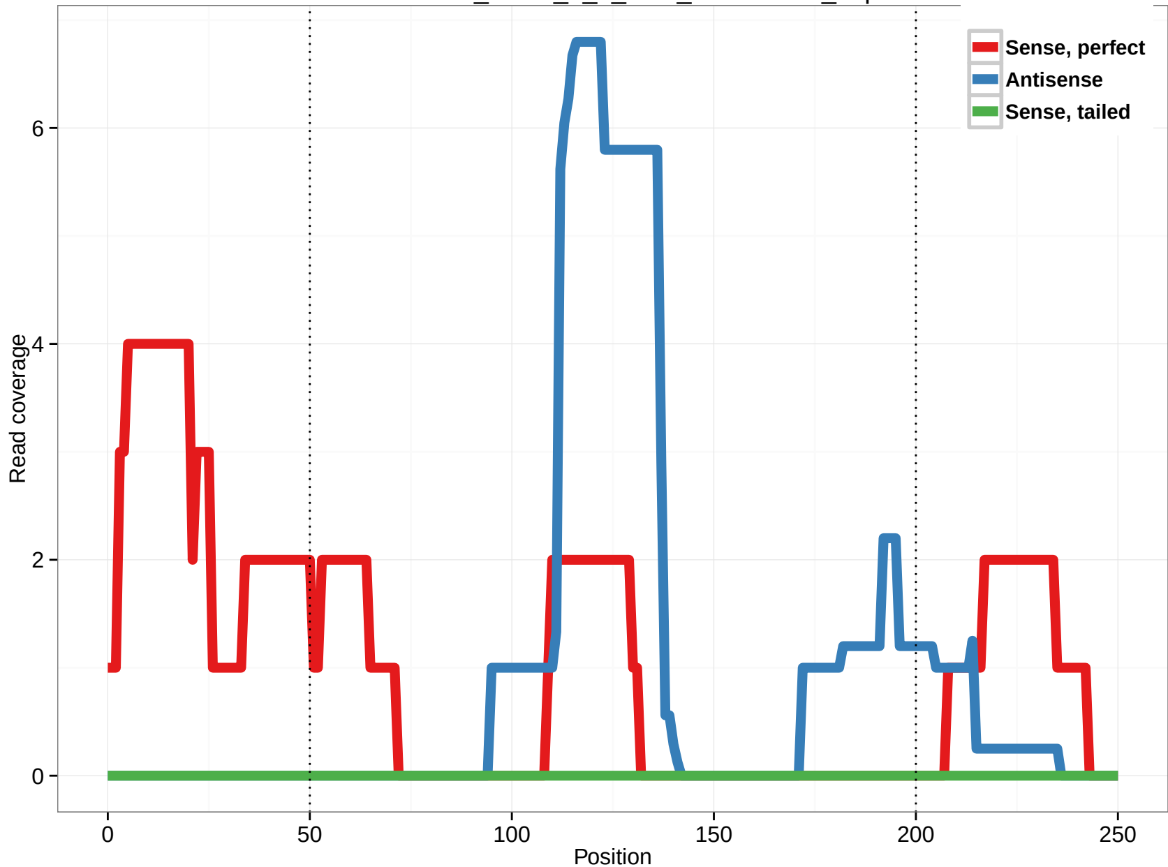
uc011ddi.1_intron_1_0_chr5_154242956_f.5p
