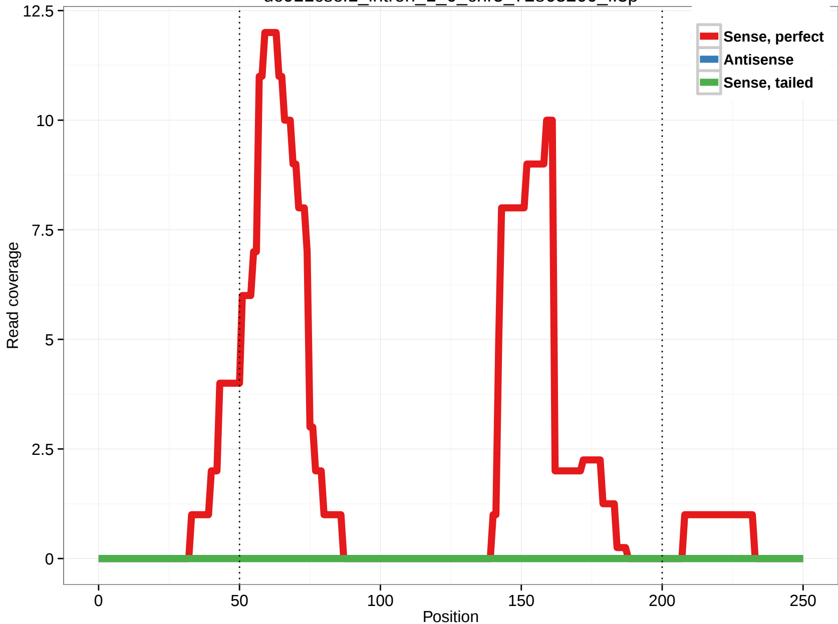
uc011cso.1_intron_1_0_chr5_72863260_f.3p
