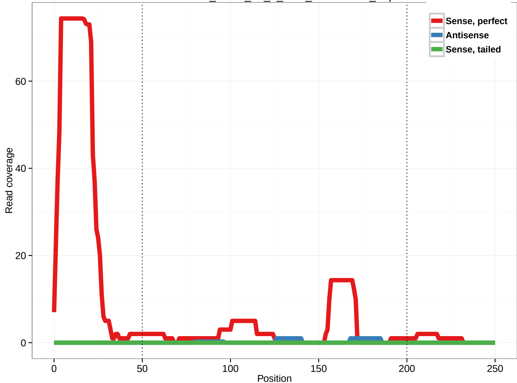
uc011cfo.1_intron_10_0_chr4_109681065_r.5p
