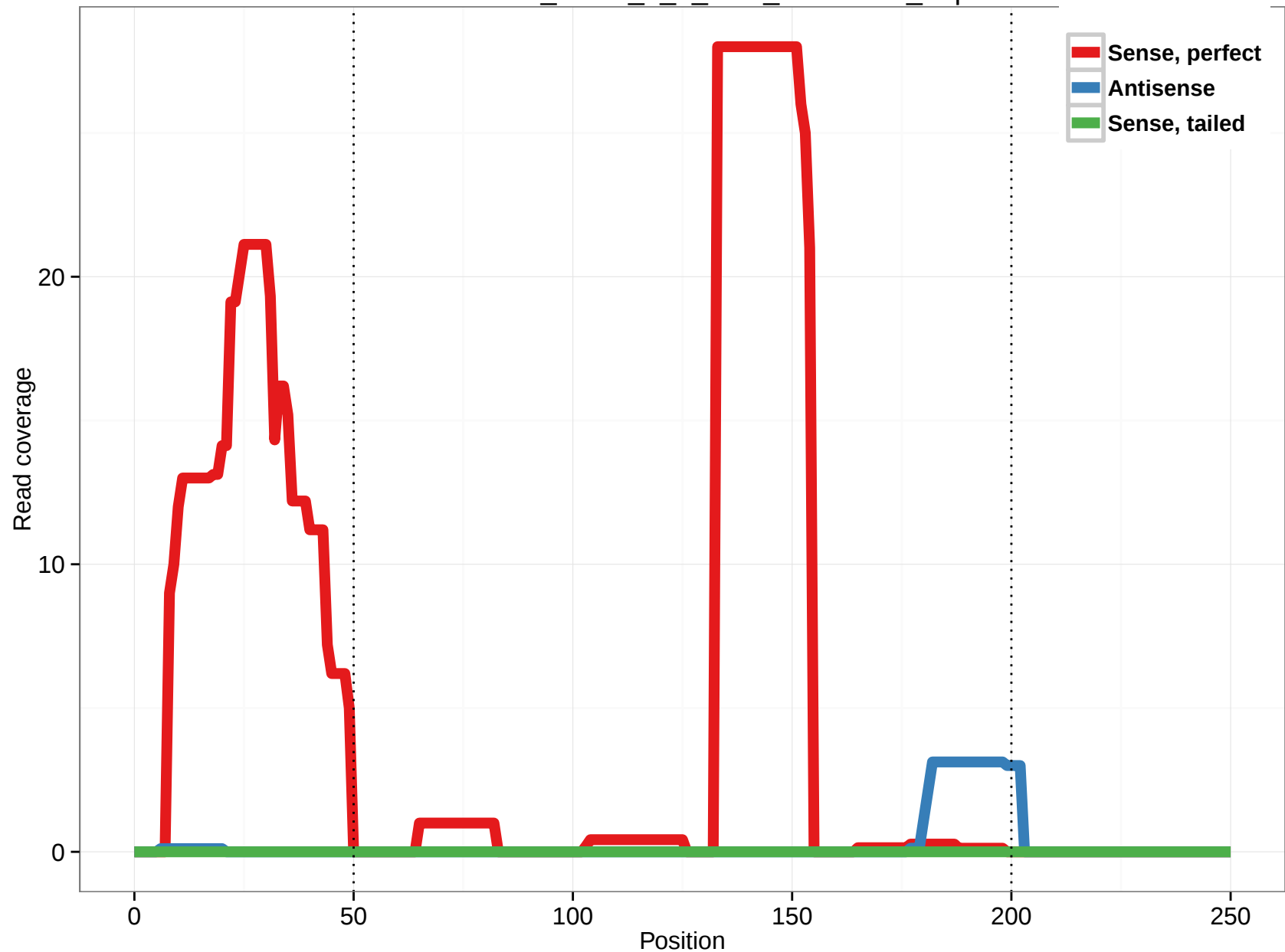
uc011caz.1_intron_3_0_chr4_71691963_r.5p
