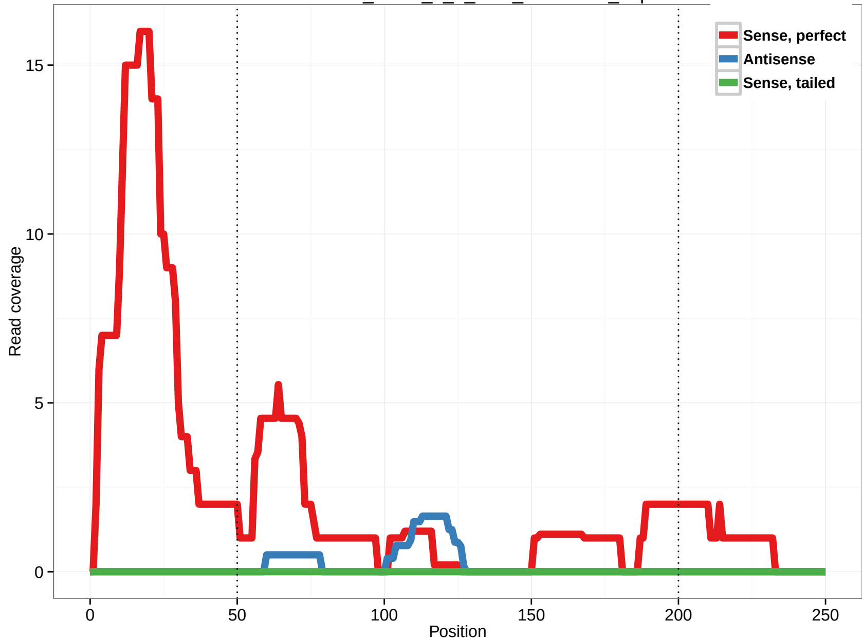
uc011bzo.1_intron_0_0_chr4_52709909_f.5p
