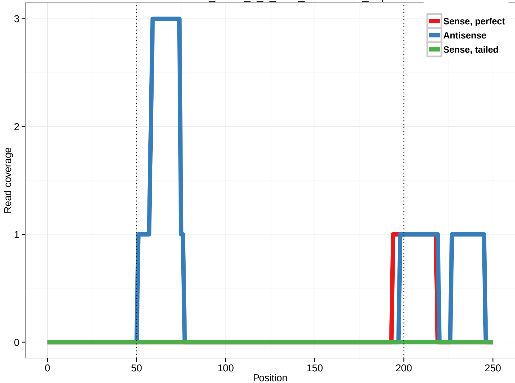
uc011bui.1_intron_0_0_chr3_197476522_f.3p
