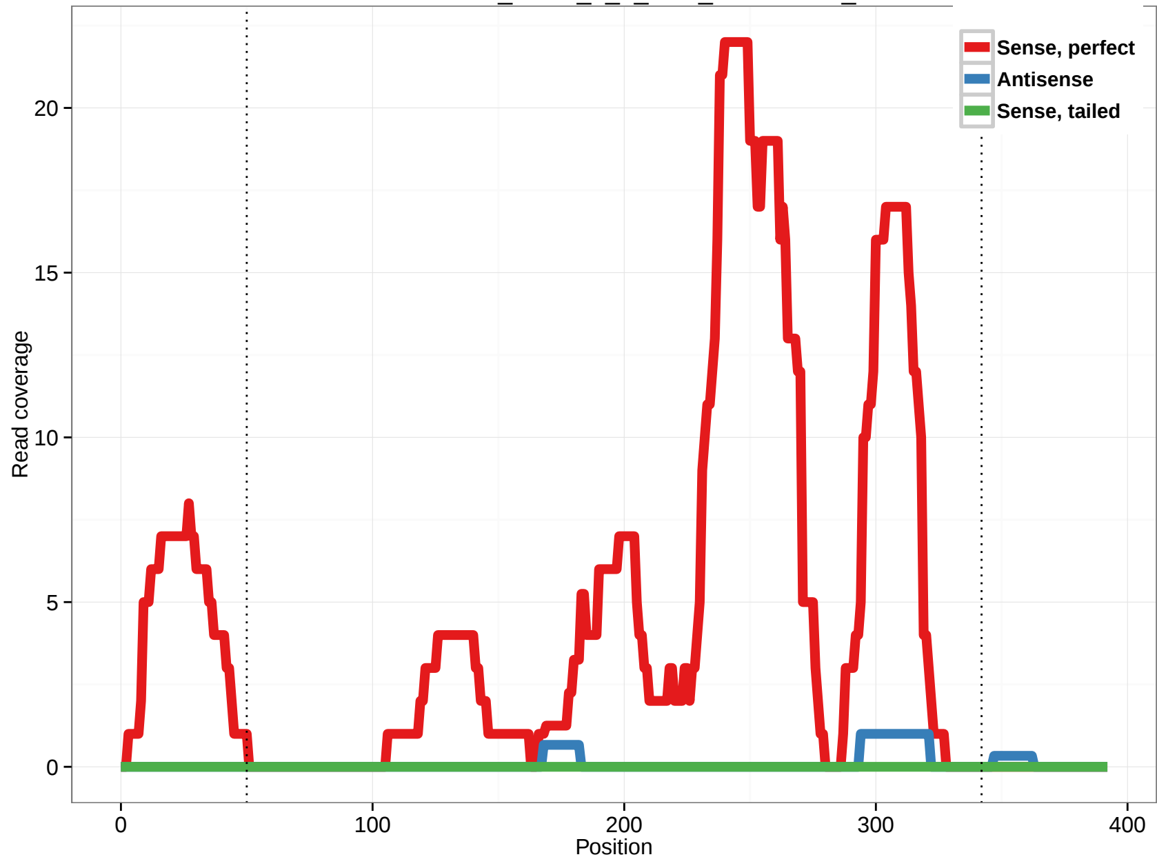
uc011boa.1_intron_0_0_chr3_151056048_r
