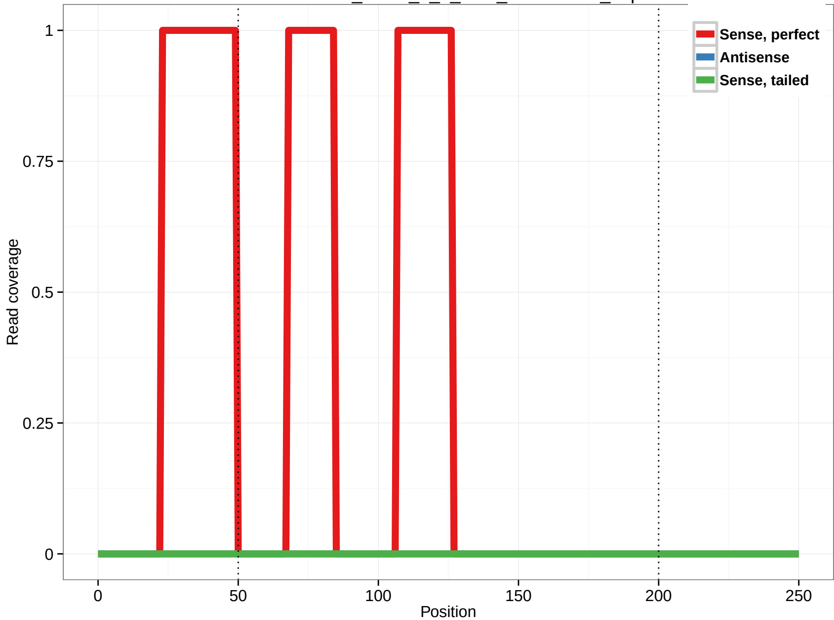
uc011bnz.1_intron_5_0_chr3_150876587_f.5p
