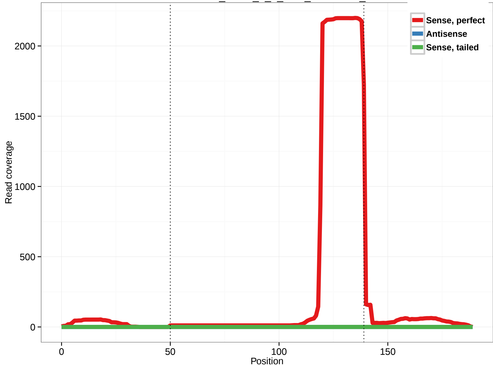
uc011bei.1_intron_1_0_chr3_52740720_f
