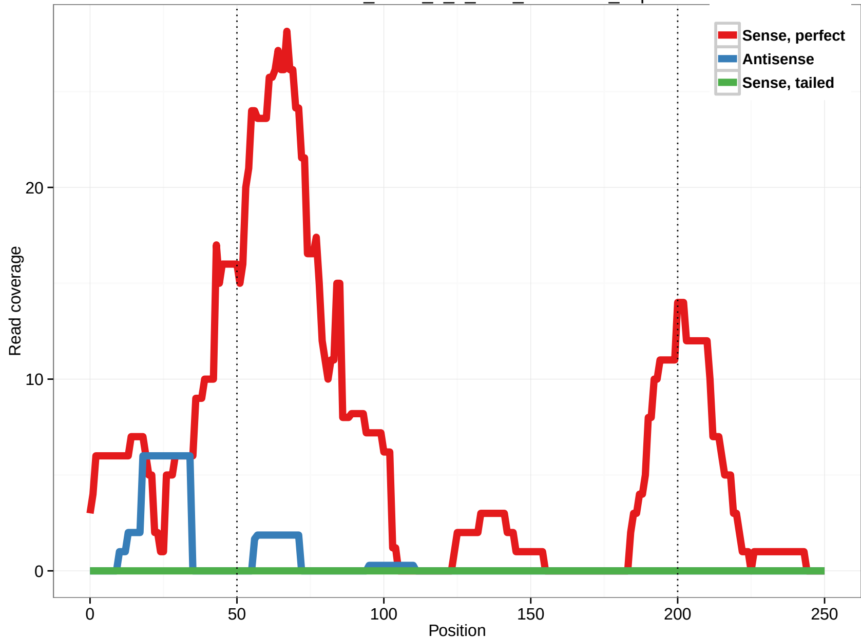
uc011beh.1_intron_0_0_chr3_52720122_f.5p
