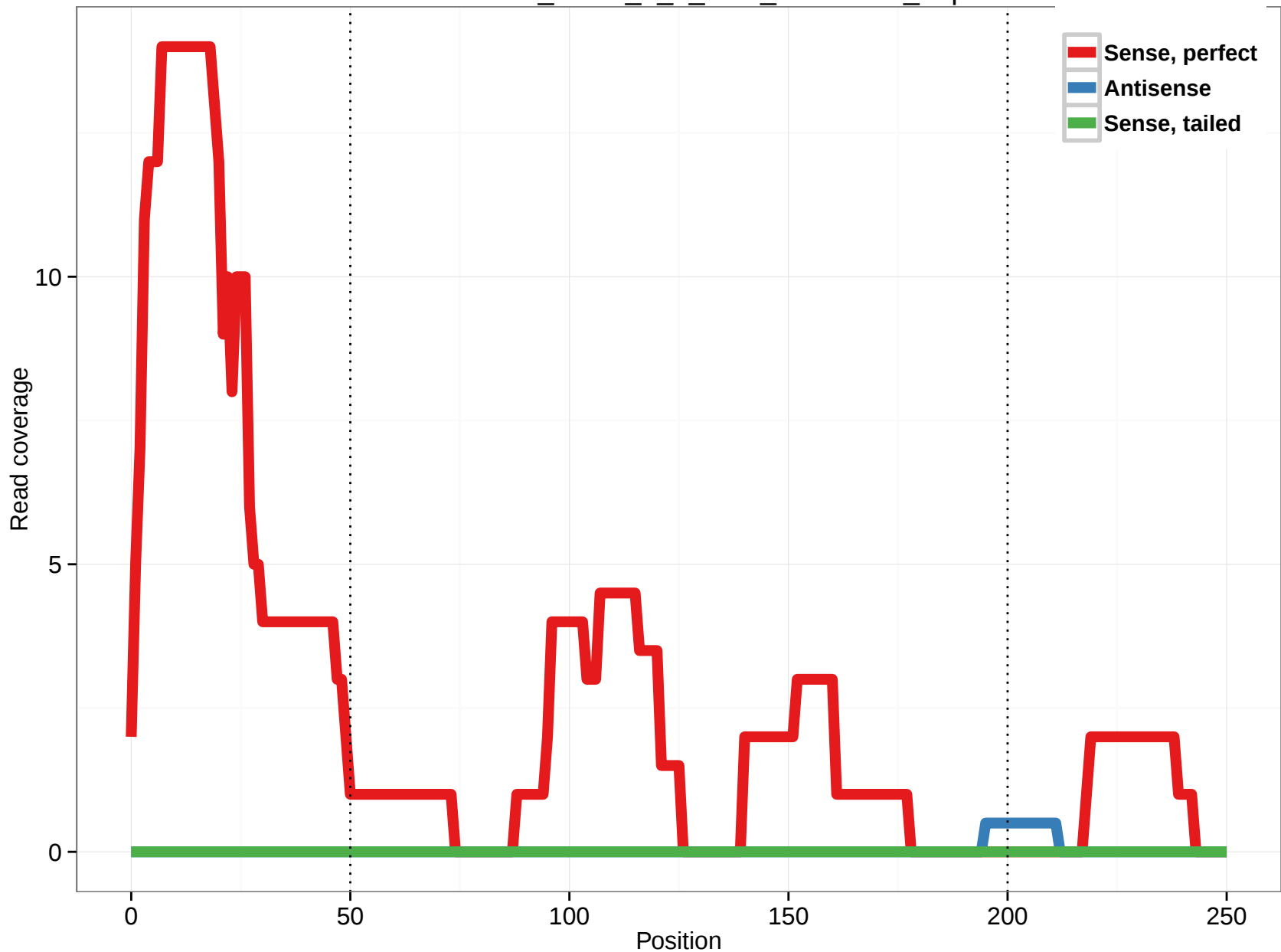
uc011bbc.1_intron_0_0_chr3_47629797_r.5p
