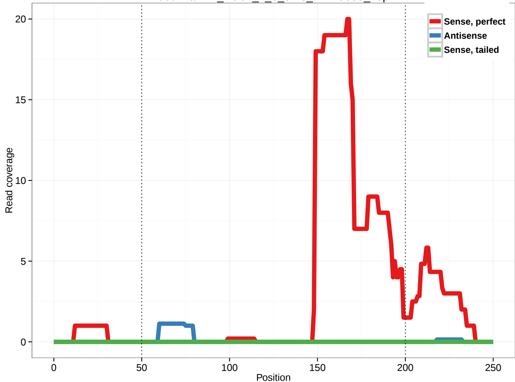
uc011azh.1_intron_4_0_chr3_42229638_f.3p
