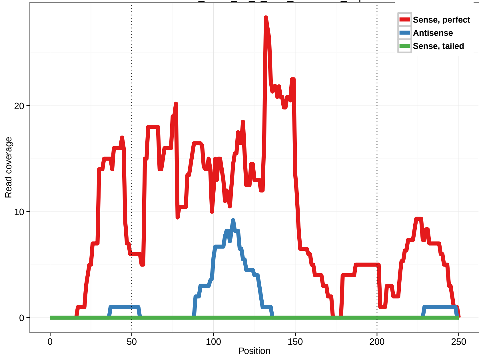
uc011avz.1_intron_26_0_chr3_15836814_r.5p
