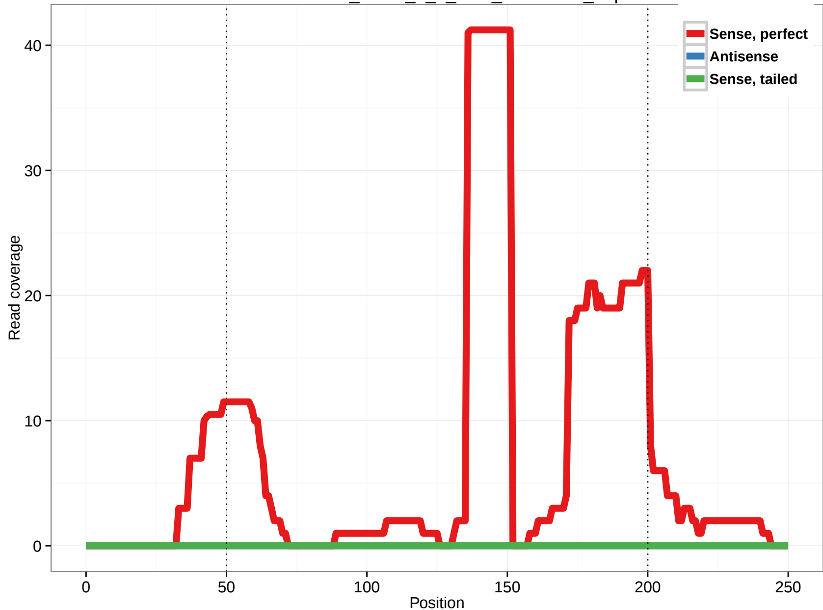
uc011avm.1_intron_0_0_chr3_15091443_r.3p
