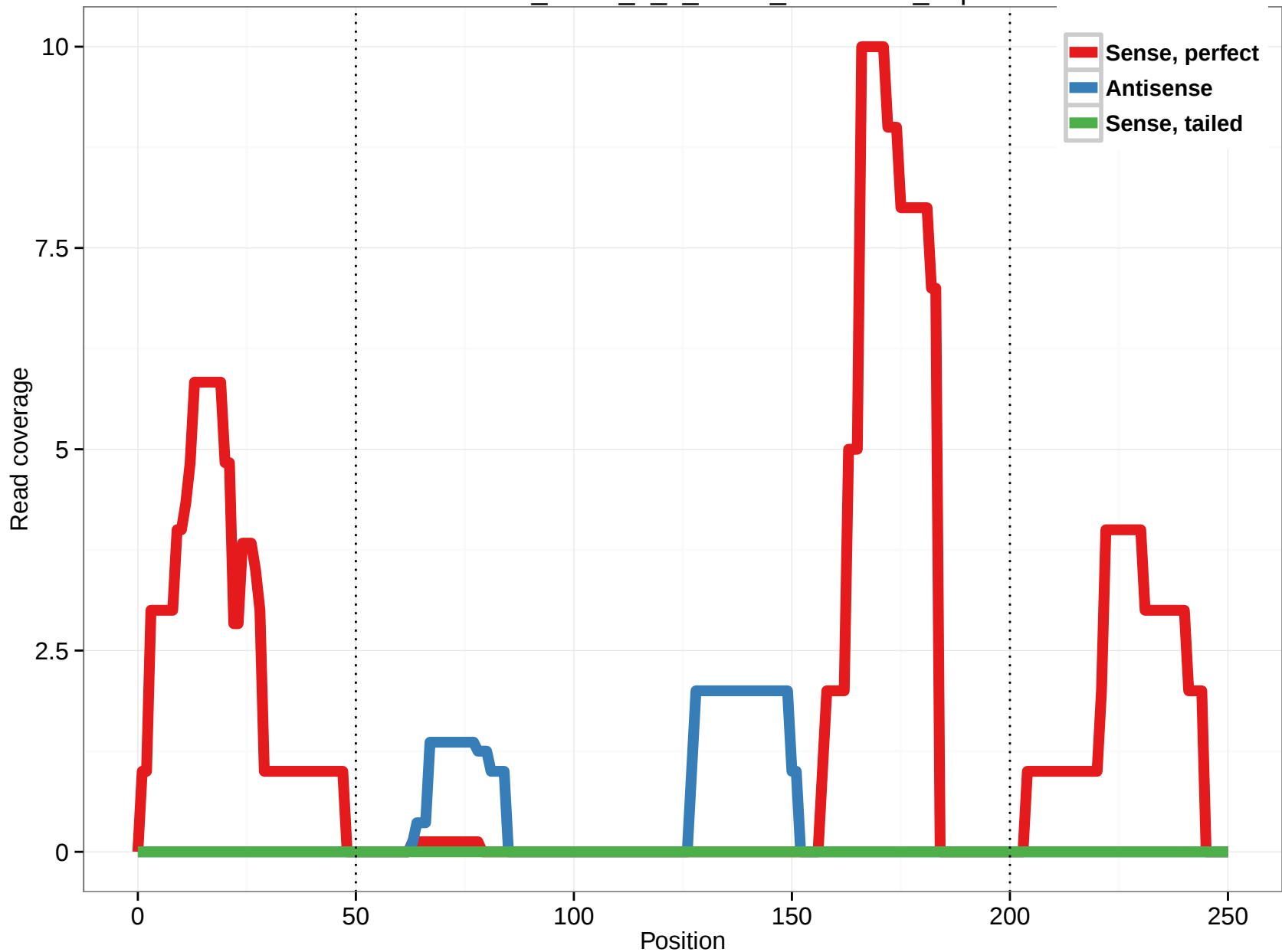
uc011arb.1_intron_0_0_chr22_46731744_f.5p
