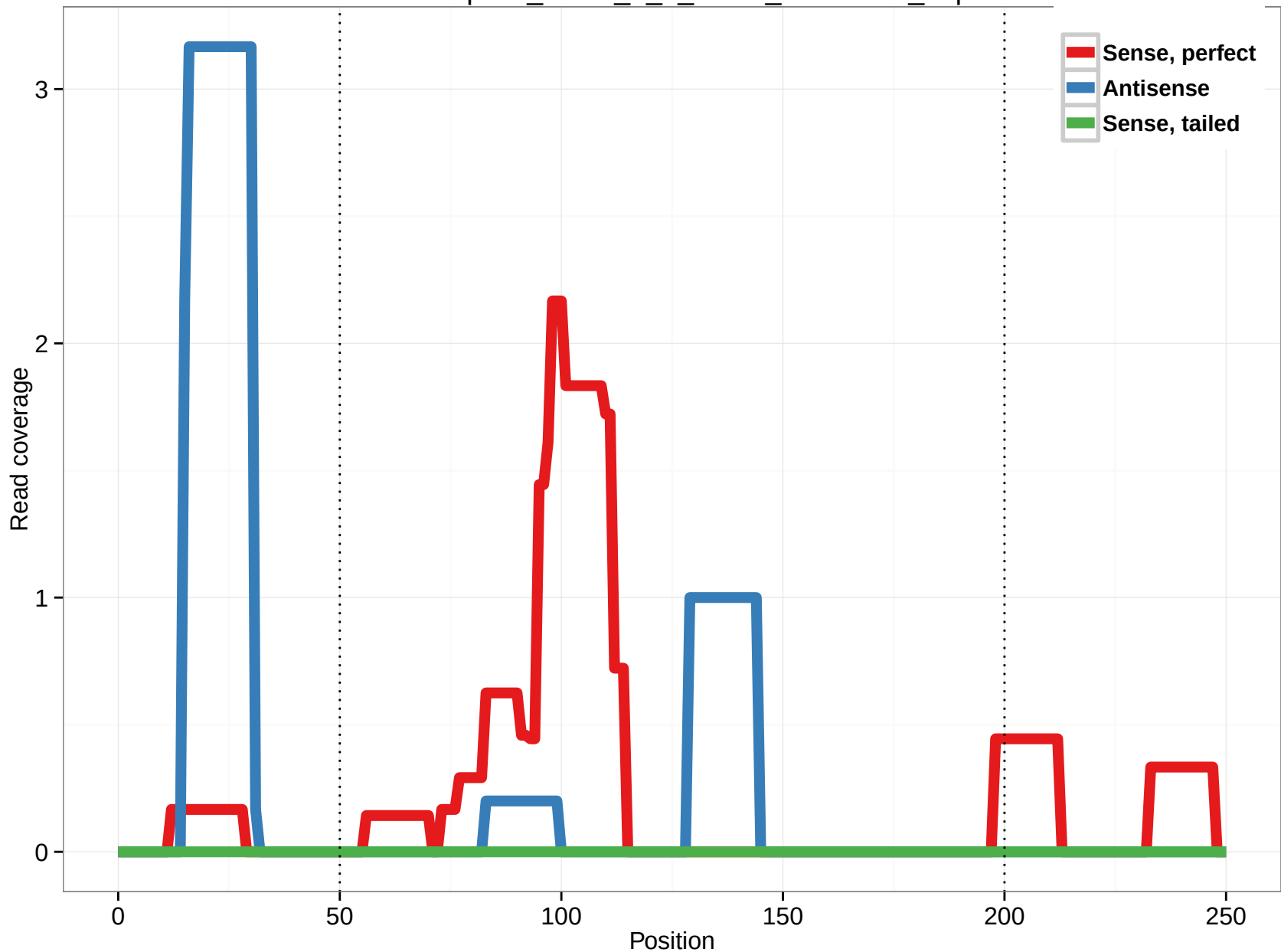
uc011apw.1_intron_0_0_chr22_43808165_f.5p
