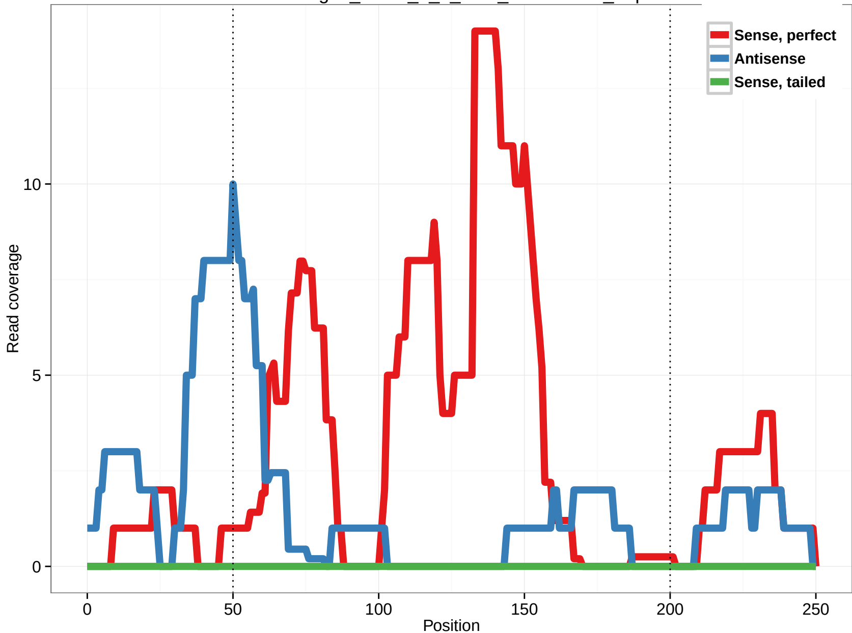
uc010zgf.1_intron_7_0_chr2_191390105_r.5p
