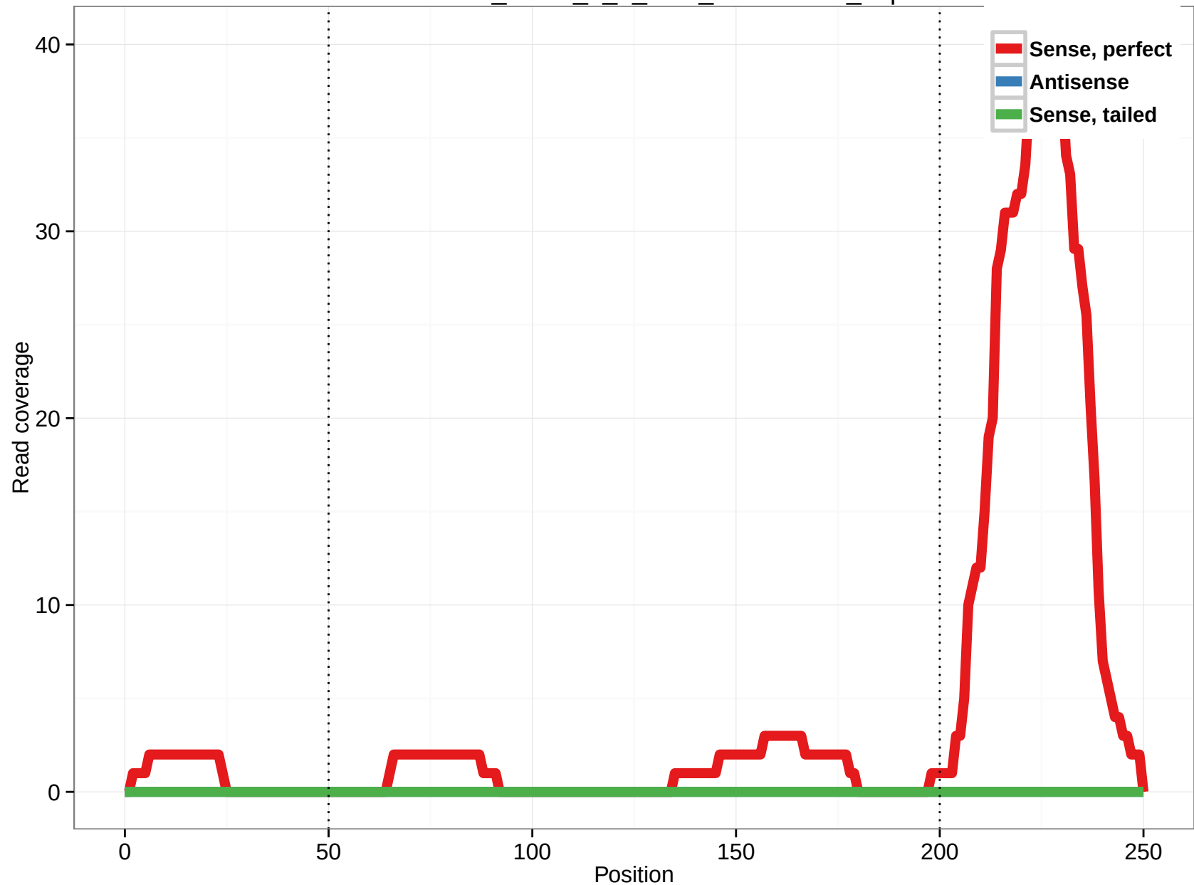
uc010zdi.1_intron_3_0_chr2_170734148_f.3p
