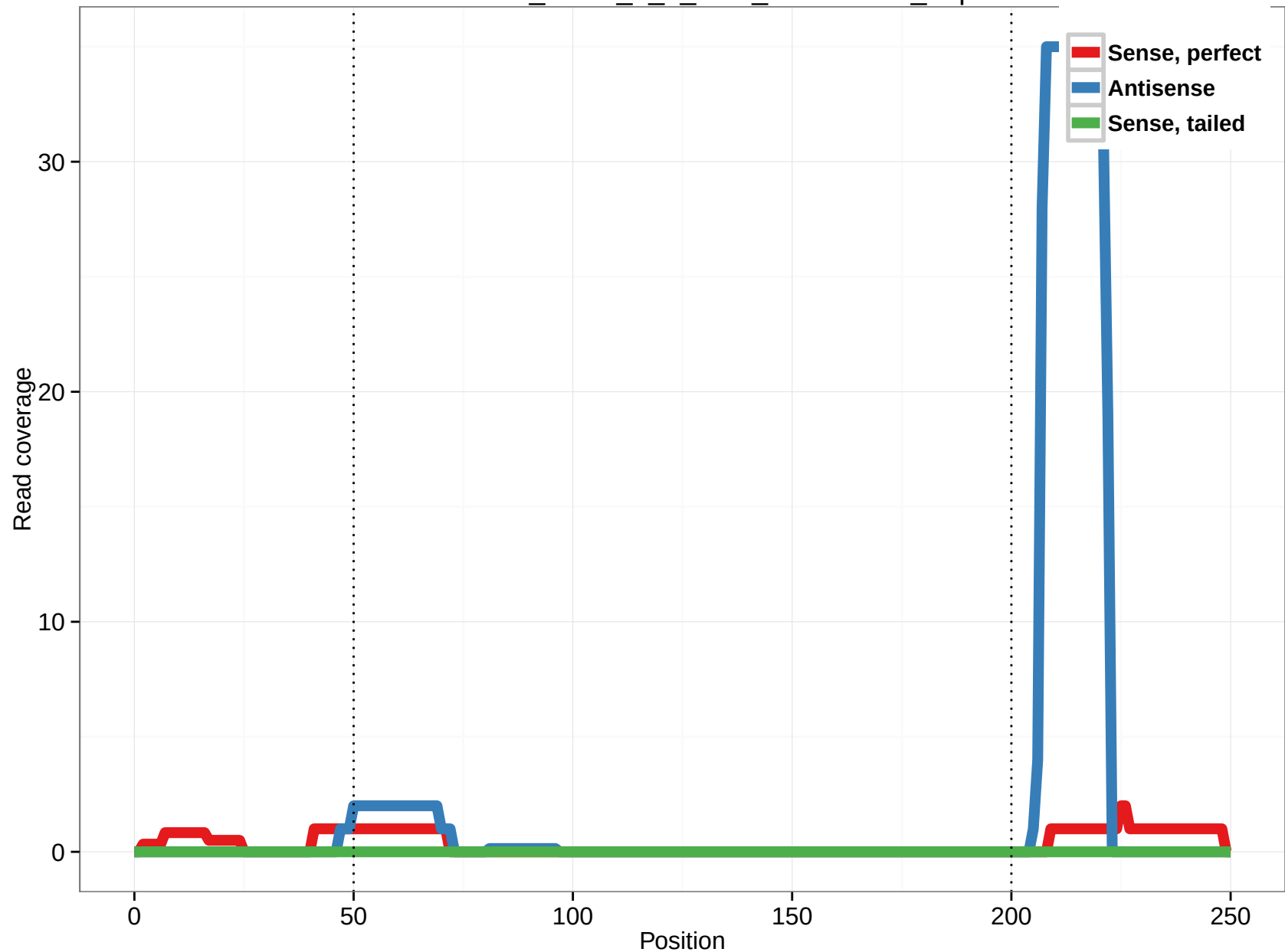
uc010zdf.1_intron_8_0_chr2_170115728_r.3p
