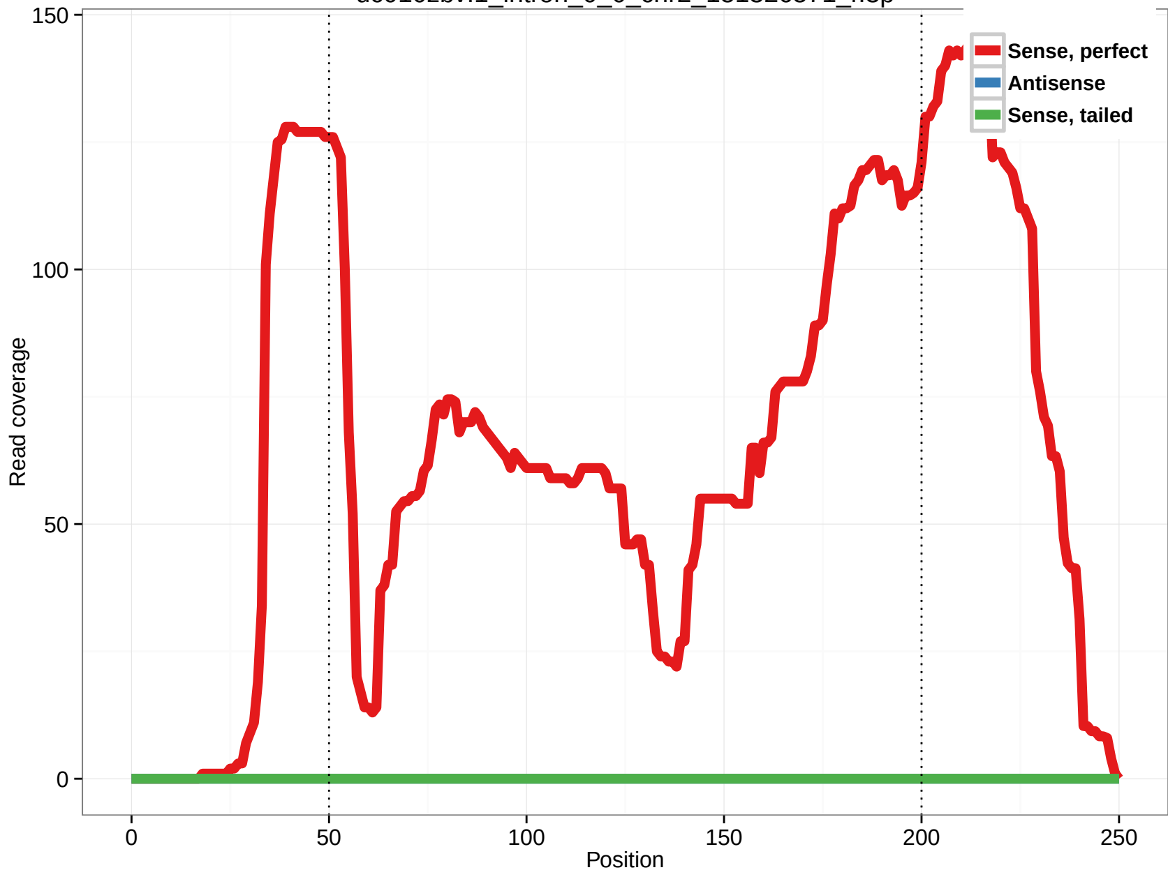
uc010zbv.1_intron_0_0_chr2_151326571_r.3p
