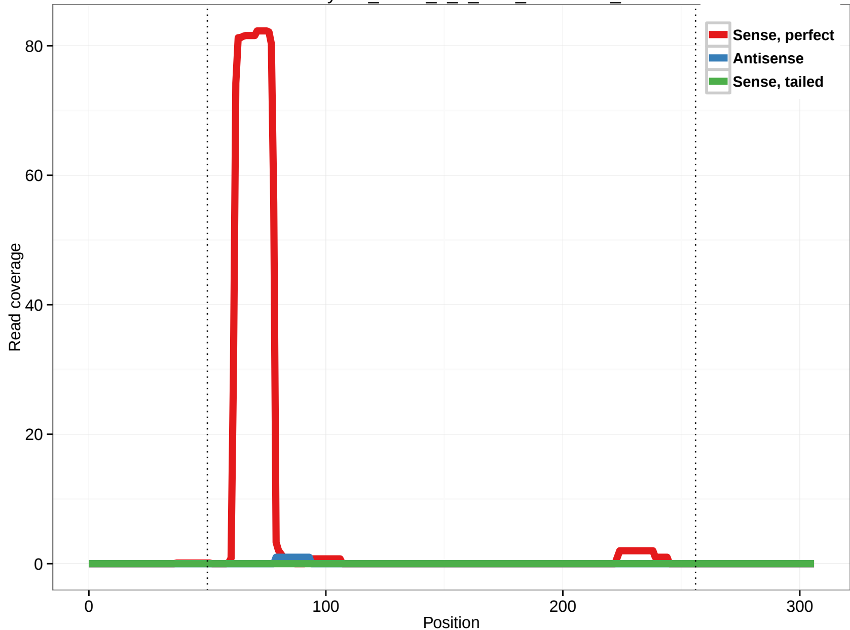
uc010ytn.1_intron_2_0_chr2_87016557_r
