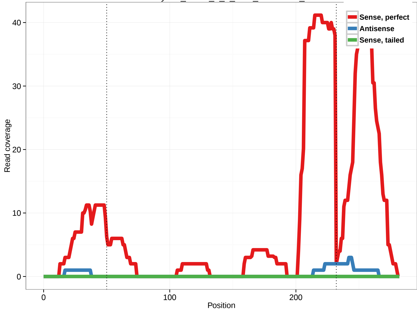
uc010ysr.1_intron_4_0_chr2_85769096_f
