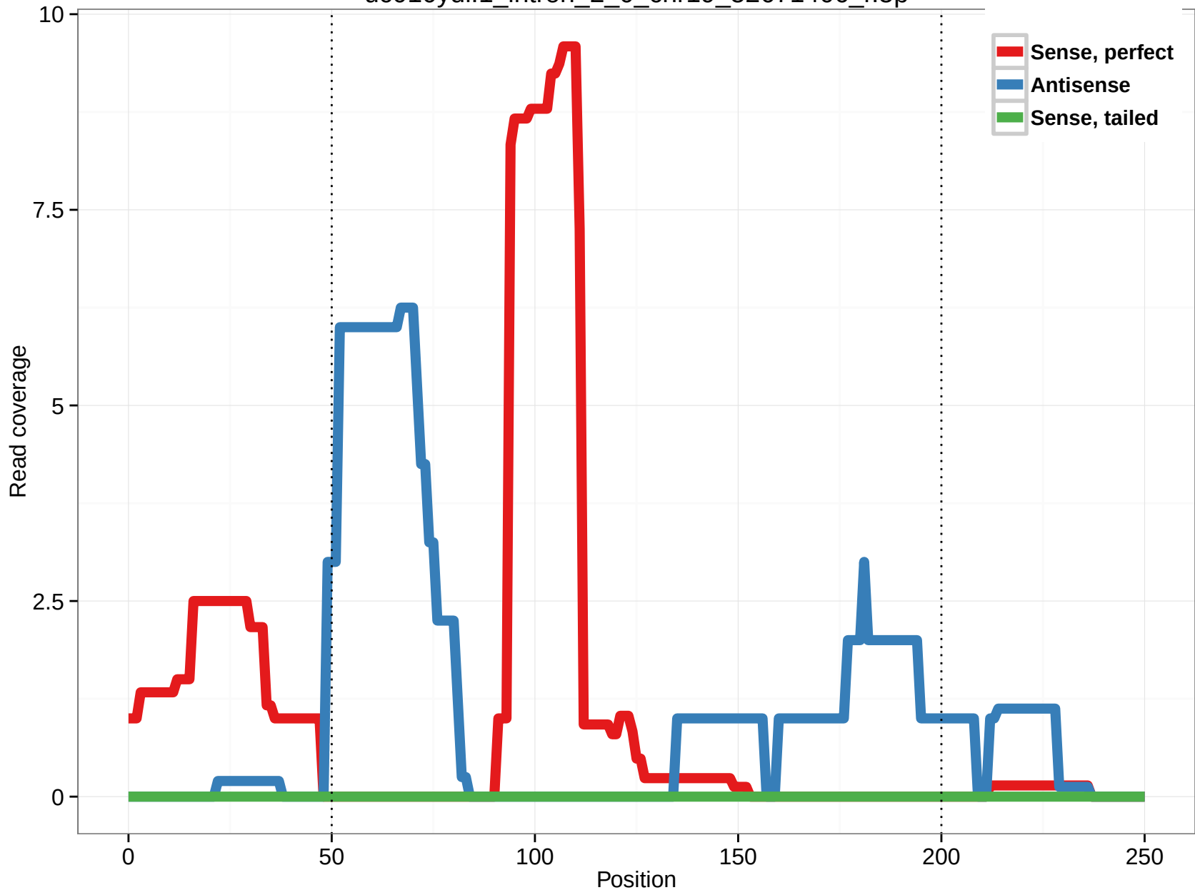
uc010ydi.1_intron_2_0_chr19_52671406_r.5p
