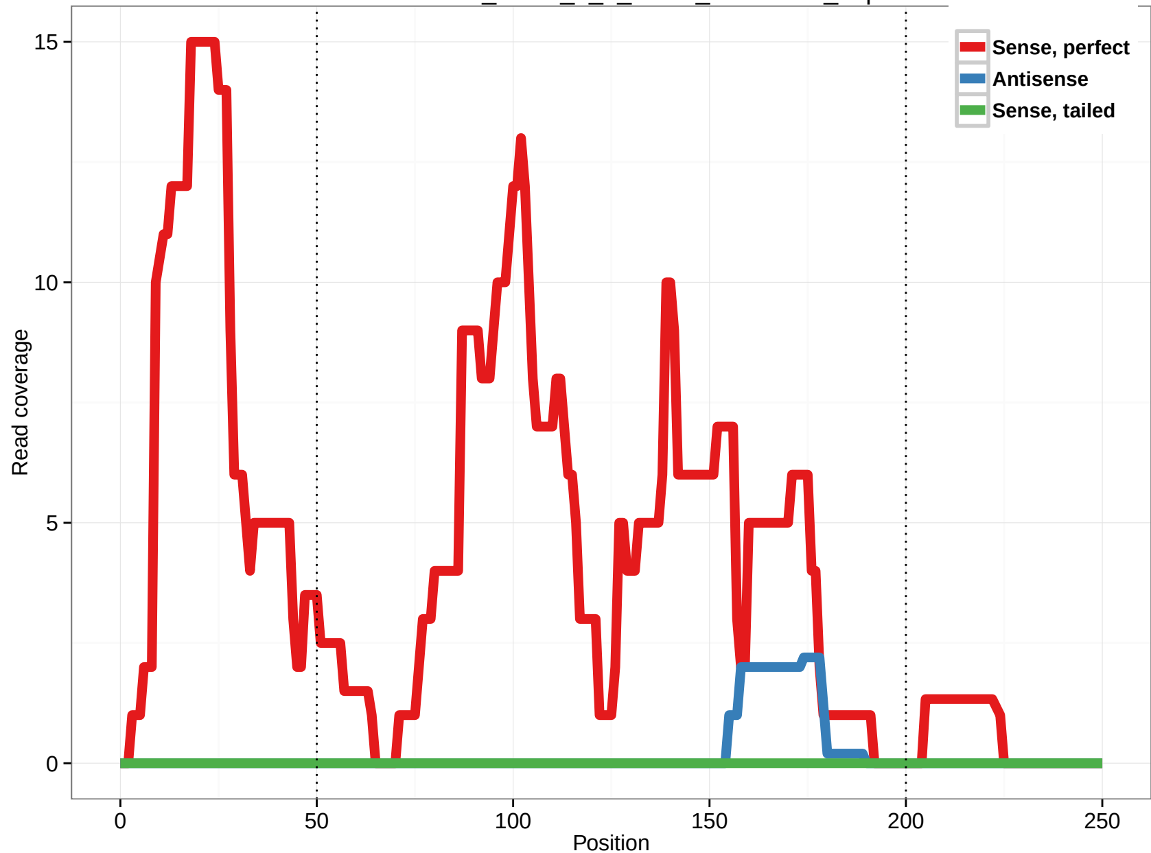
uc010xmh.1_intron_0_0_chr19_12274022_f.5p
